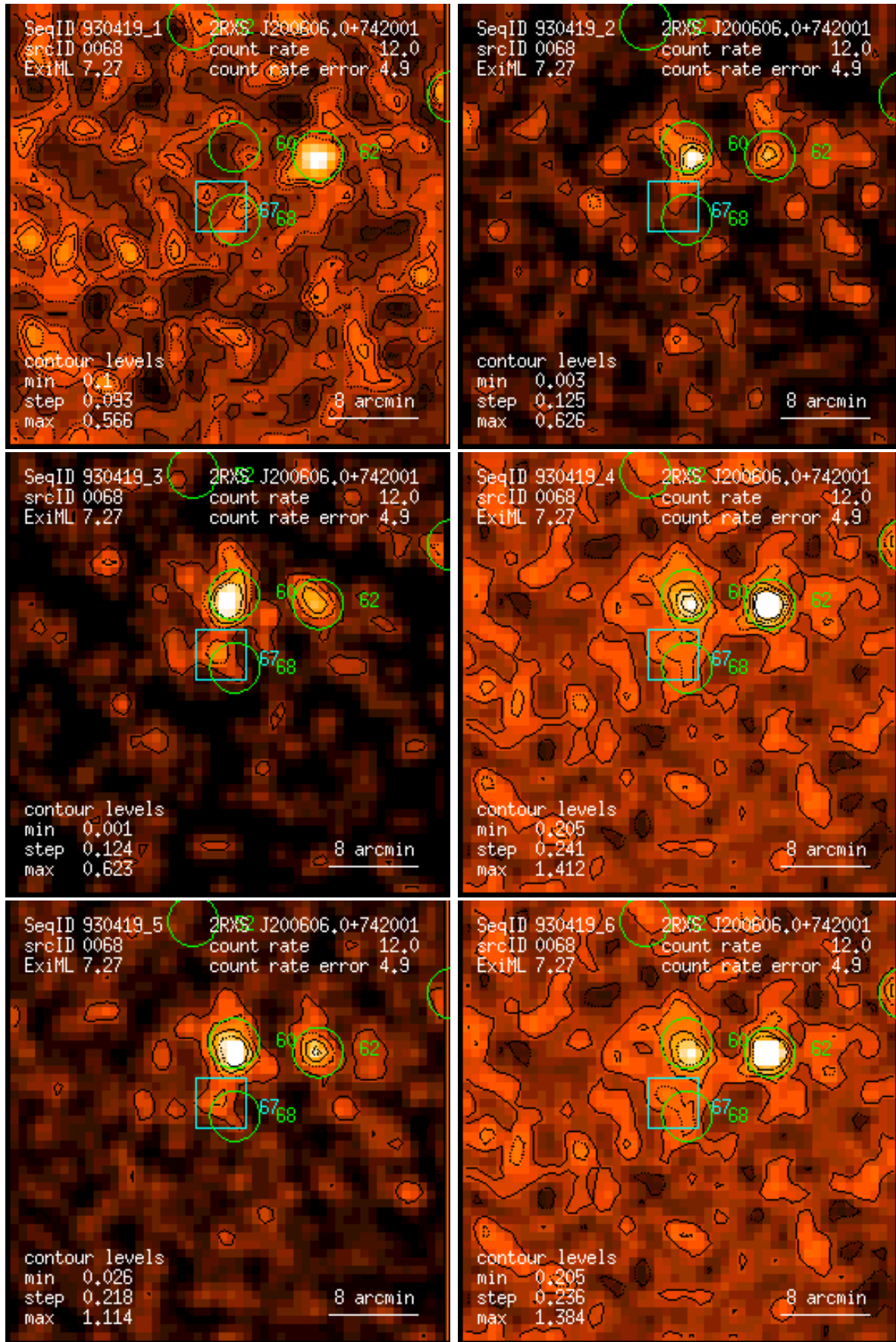
Figure 68: RASS 930419: detection 0068: band rate images, Gaussian filter: (1) PSPC channels 11 – 41, (2) 52 – 90, (3) 91 – 201, (4) 11 – 235, (5) 52 – 201, (6) 11 – 201. Broad band rates in counts/ks. Band rate contour levels in counts/ks/arcmin 2 .
