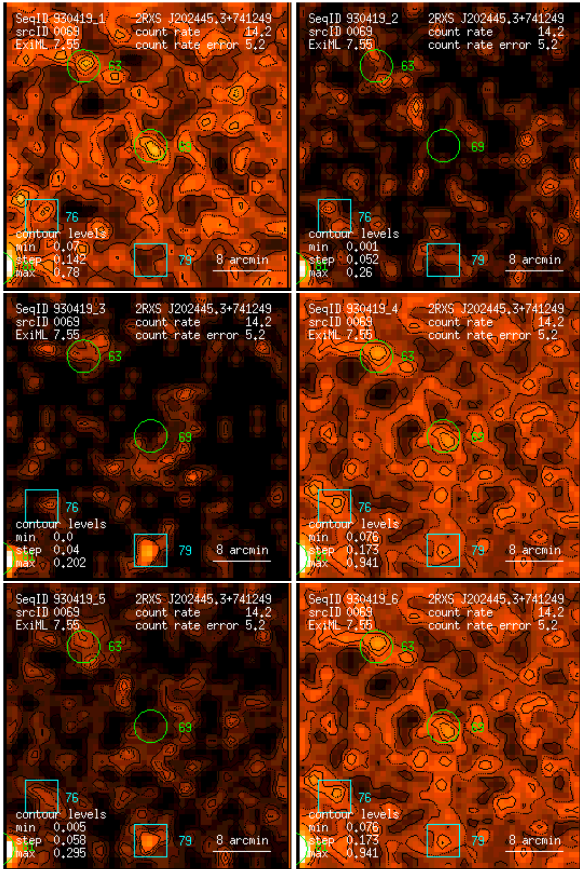
Figure 69: RASS 930419: detection 0069: band rate images, Gaussian filter: (1) PSPC channels 11 – 41, (2) 52 – 90, (3) 91 – 201, (4) 11 – 235, (5) 52 – 201, (6) 11 – 201. Broad band rates in counts/ks. Band rate contour levels in counts/ks/arcmin 2 .
