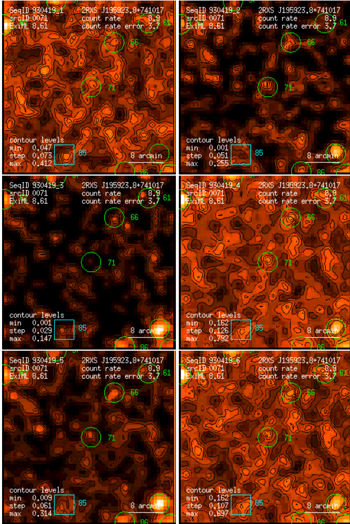
Figure 71: RASS 930419: detection 0071: band rate images, Gaussian filter: (1) PSPC channels 11 – 41, (2) 52 – 90, (3) 91 – 201, (4) 11 – 235, (5) 52 – 201, (6) 11 – 201. Broad band rates in counts/ks. Band rate contour levels in counts/ks/arcmin 2 .
