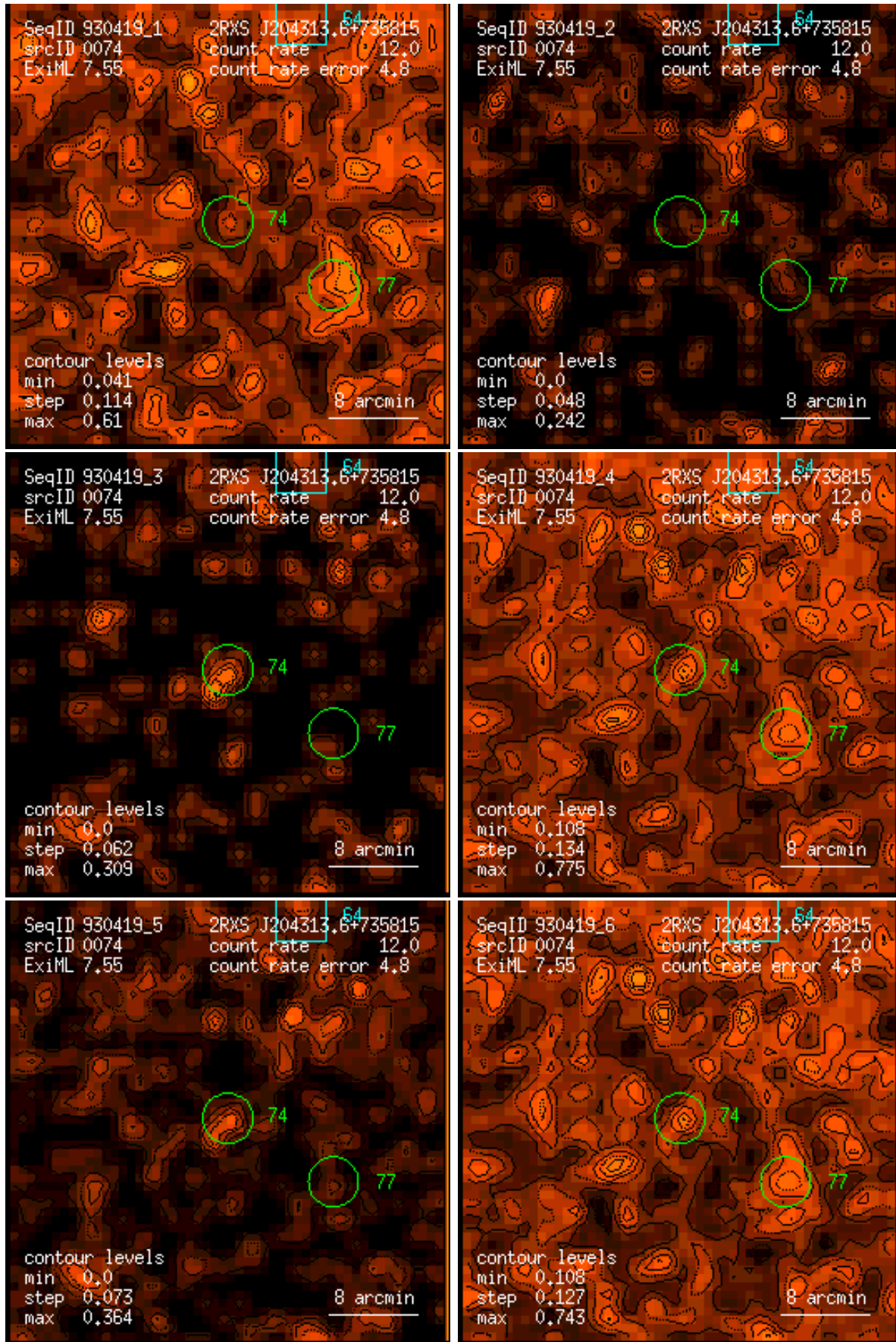
Figure 74: RASS 930419: detection 0074: band rate images, Gaussian filter: (1) PSPC channels 11 – 41, (2) 52 – 90, (3) 91 – 201, (4) 11 – 235, (5) 52 – 201, (6) 11 – 201. Broad band rates in counts/ks. Band rate contour levels in counts/ks/arcmin 2 .
