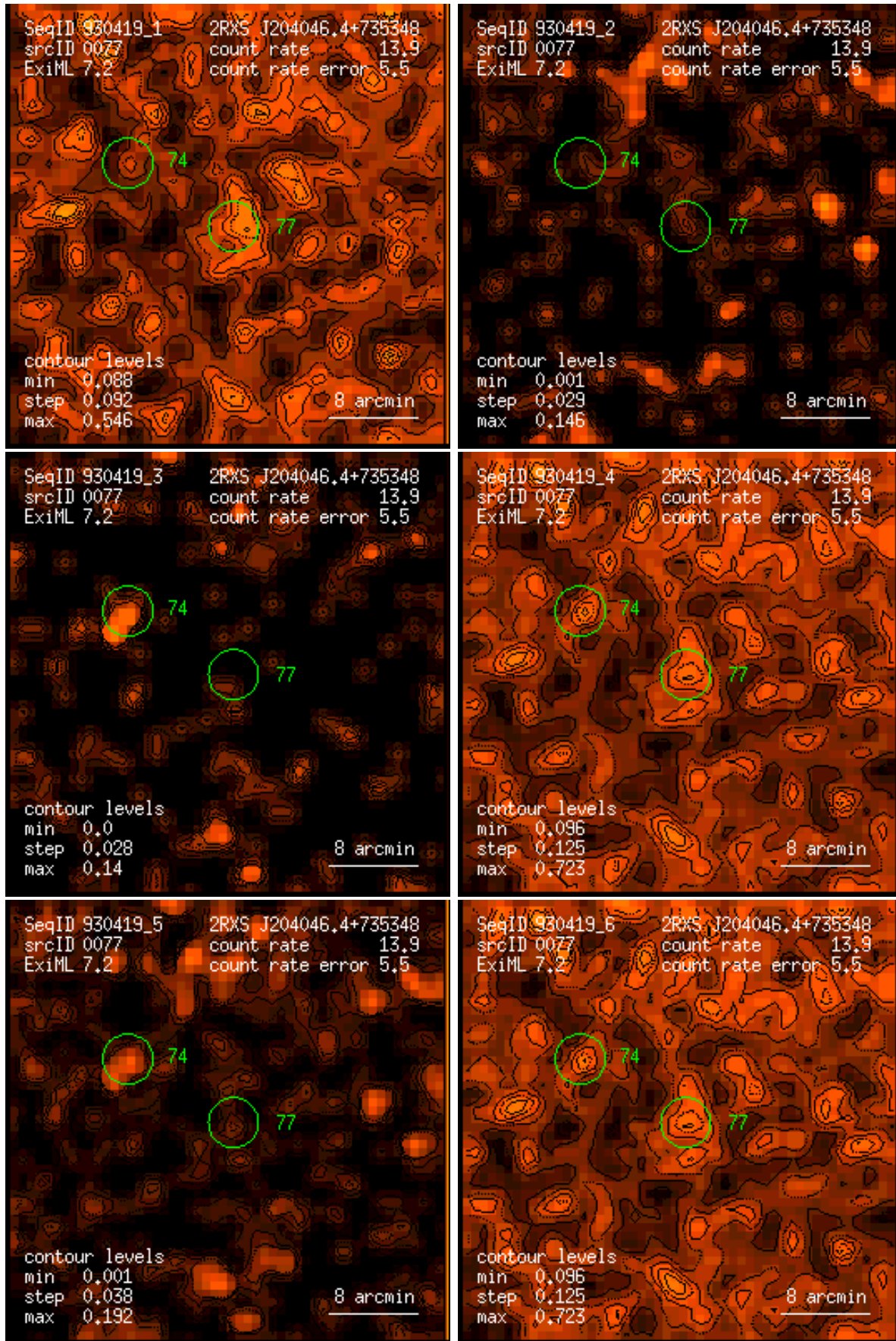
Figure 77: RASS 930419: detection 0077: band rate images, Gaussian filter: (1) PSPC channels 11 – 41, (2) 52 – 90, (3) 91 – 201, (4) 11 – 235, (5) 52 – 201, (6) 11 – 201. Broad band rates in counts/ks. Band rate contour levels in counts/ks/arcmin 2 .
