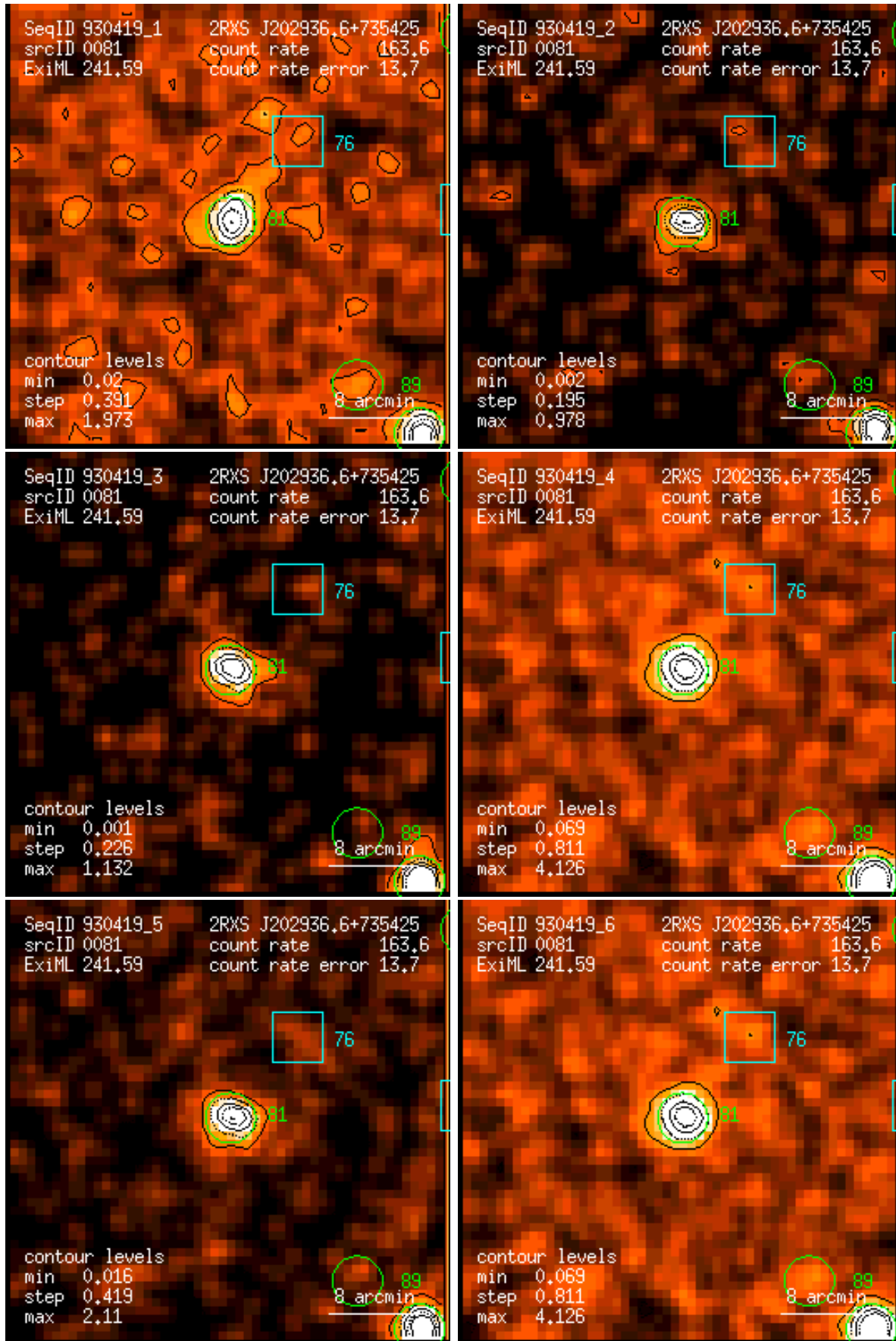
Figure 81: RASS 930419: detection 0081: band rate images, Gaussian filter: (1) PSPC channels 11 – 41, (2) 52 – 90, (3) 91 – 201, (4) 11 – 235, (5) 52 – 201, (6) 11 – 201. Broad band rates in counts/ks. Band rate contour levels in counts/ks/arcmin 2 .
