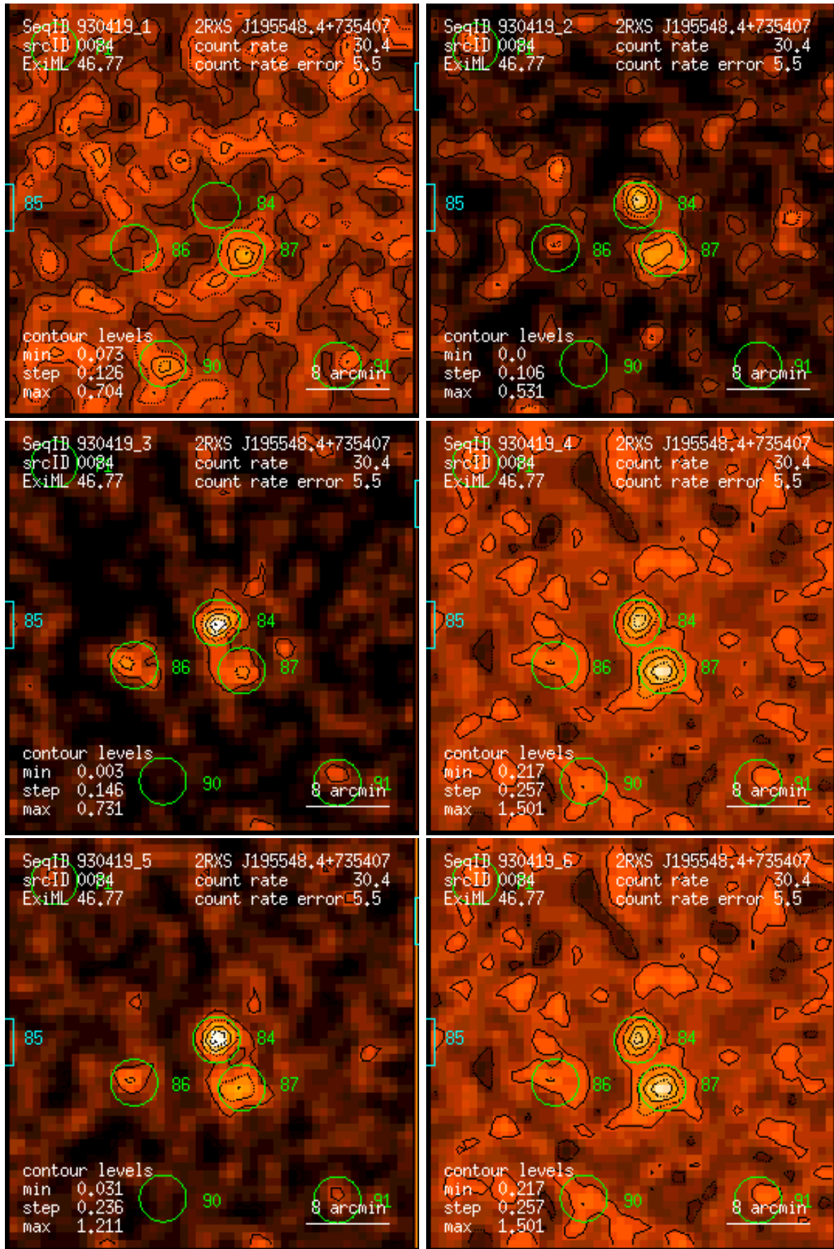
Figure 84: RASS 930419: detection 0084: band rate images, Gaussian filter: (1) PSPC channels 11 – 41, (2) 52 – 90, (3) 91 – 201, (4) 11 – 235, (5) 52 – 201, (6) 11 – 201. Broad band rates in counts/ks. Band rate contour levels in counts/ks/arcmin 2 .
