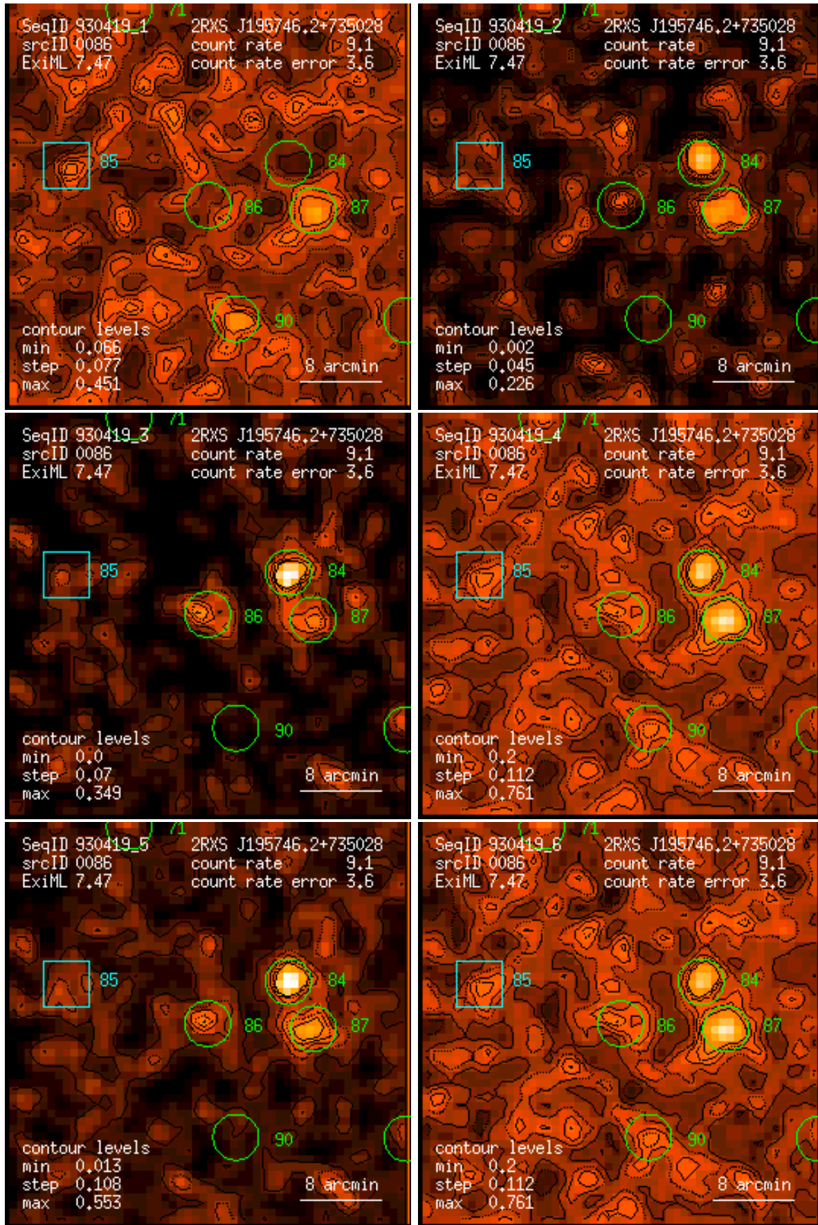
Figure 86: RASS 930419: detection 0086: band rate images, Gaussian filter: (1) PSPC channels 11 – 41, (2) 52 – 90, (3) 91 – 201, (4) 11 – 235, (5) 52 – 201, (6) 11 – 201. Broad band rates in counts/ks. Band rate contour levels in counts/ks/arcmin 2 .
