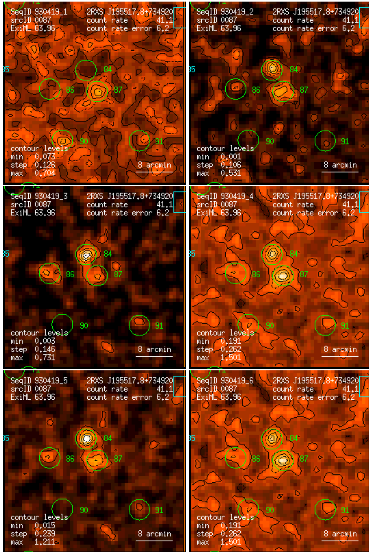
Figure 87: RASS 930419: detection 0087: band rate images, Gaussian filter: (1) PSPC channels 11 – 41, (2) 52 – 90, (3) 91 – 201, (4) 11 – 235, (5) 52 – 201, (6) 11 – 201. Broad band rates in counts/ks. Band rate contour levels in counts/ks/arcmin 2 .
