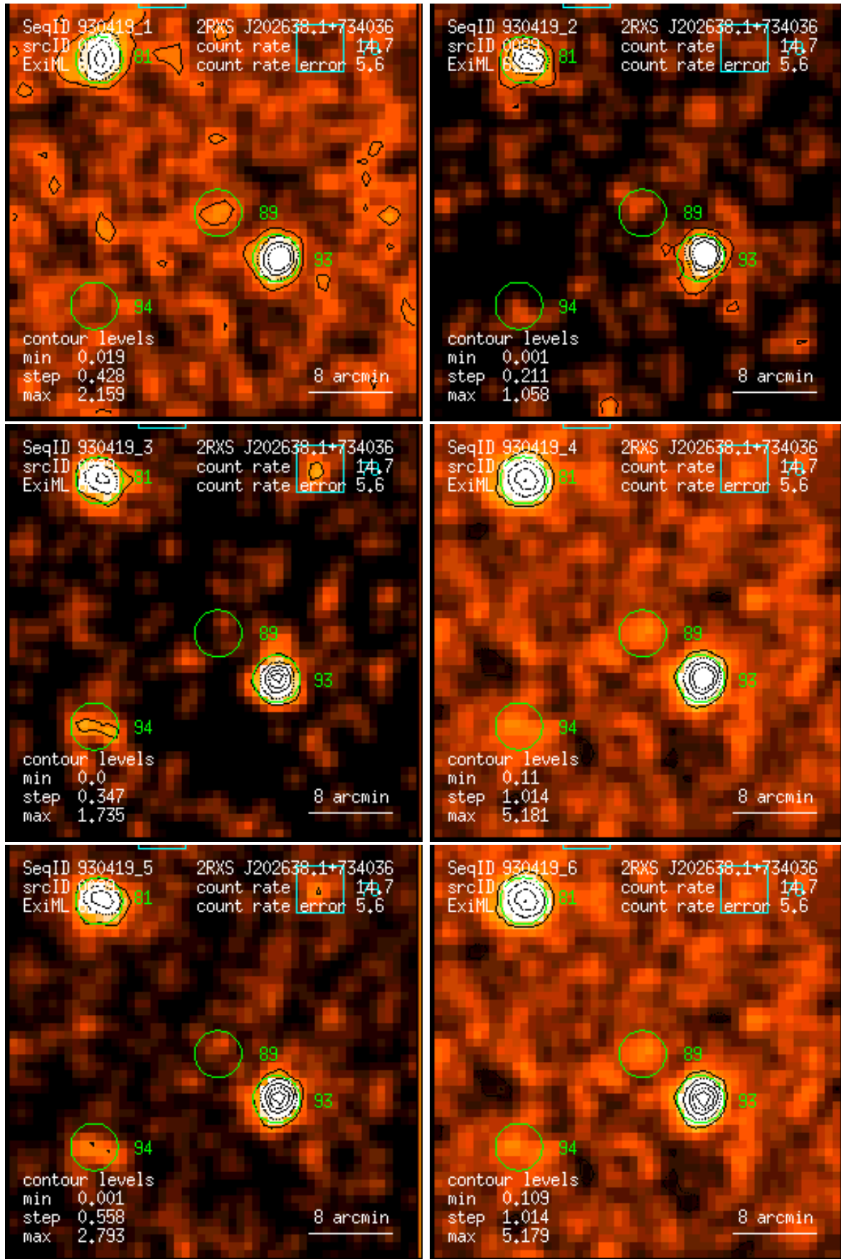
Figure 89: RASS 930419: detection 0089: band rate images, Gaussian filter: (1) PSPC channels 11 – 41, (2) 52 – 90, (3) 91 – 201, (4) 11 – 235, (5) 52 – 201, (6) 11 – 201. Broad band rates in counts/ks. Band rate contour levels in counts/ks/arcmin 2 .
