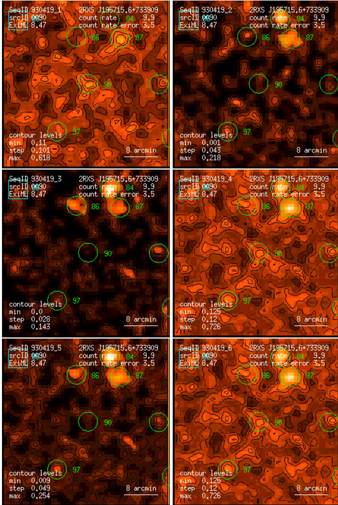
Figure 90: RASS 930419: detection 0090: band rate images, Gaussian filter: (1) PSPC channels 11 – 41, (2) 52 – 90, (3) 91 – 201, (4) 11 – 235, (5) 52 – 201, (6) 11 – 201. Broad band rates in counts/ks. Band rate contour levels in counts/ks/arcmin 2 .
