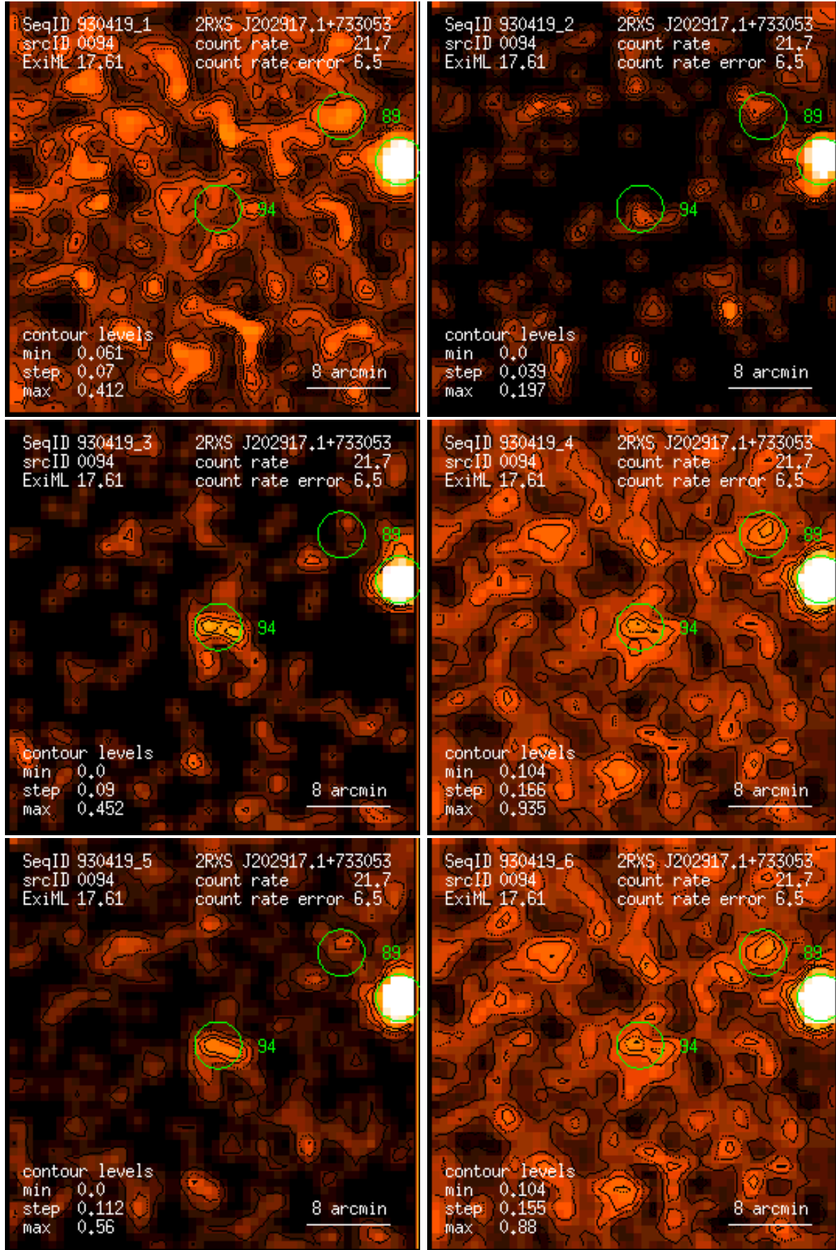
Figure 94: RASS 930419: detection 0094: band rate images, Gaussian filter: (1) PSPC channels 11 – 41, (2) 52 – 90, (3) 91 – 201, (4) 11 – 235, (5) 52 – 201, (6) 11 – 201. Broad band rates in counts/ks. Band rate contour levels in counts/ks/arcmin 2 .
