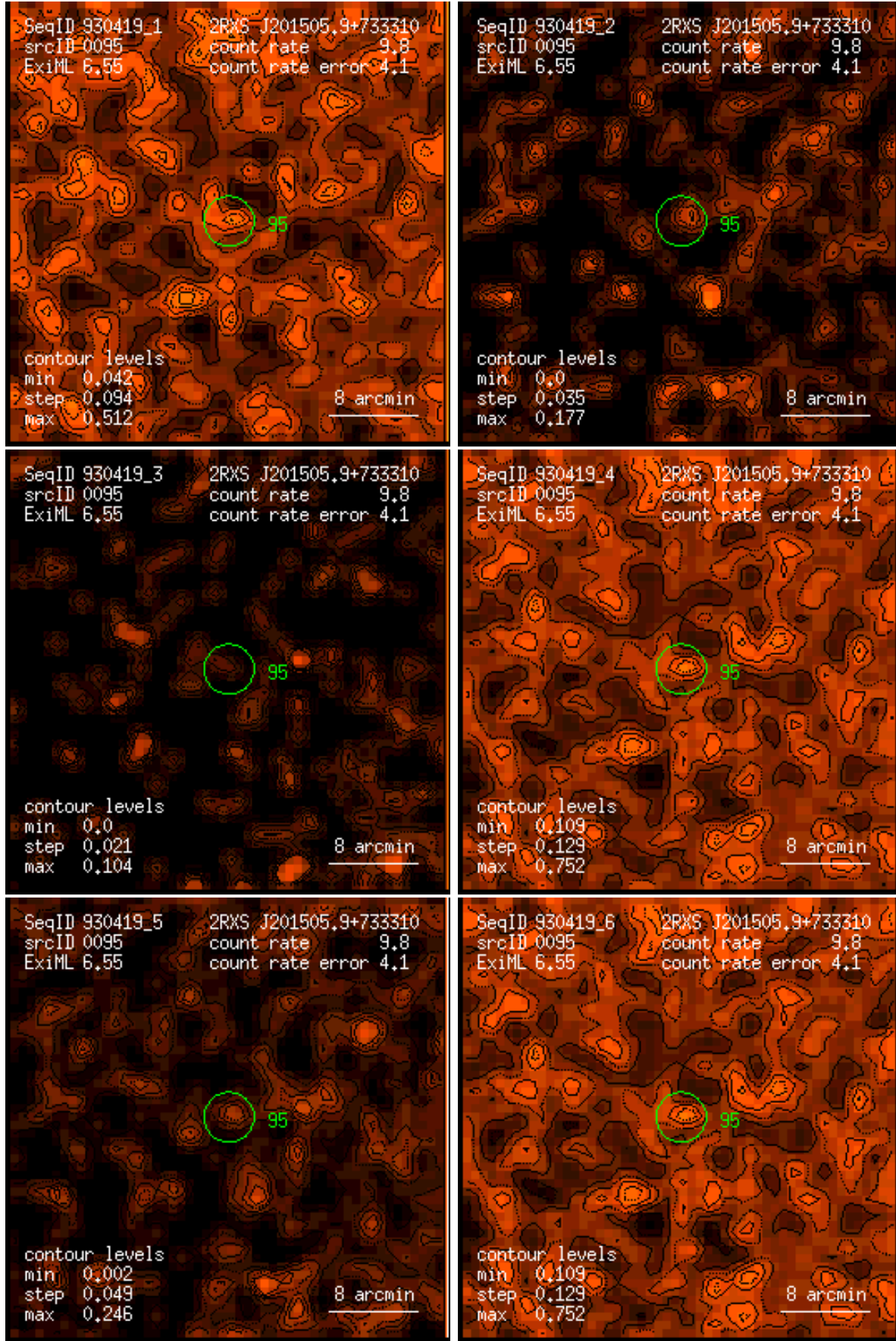
Figure 95: RASS 930419: detection 0095: band rate images, Gaussian filter: (1) PSPC channels 11 – 41, (2) 52 – 90, (3) 91 – 201, (4) 11 – 235, (5) 52 – 201, (6) 11 – 201. Broad band rates in counts/ks. Band rate contour levels in counts/ks/arcmin 2 .
