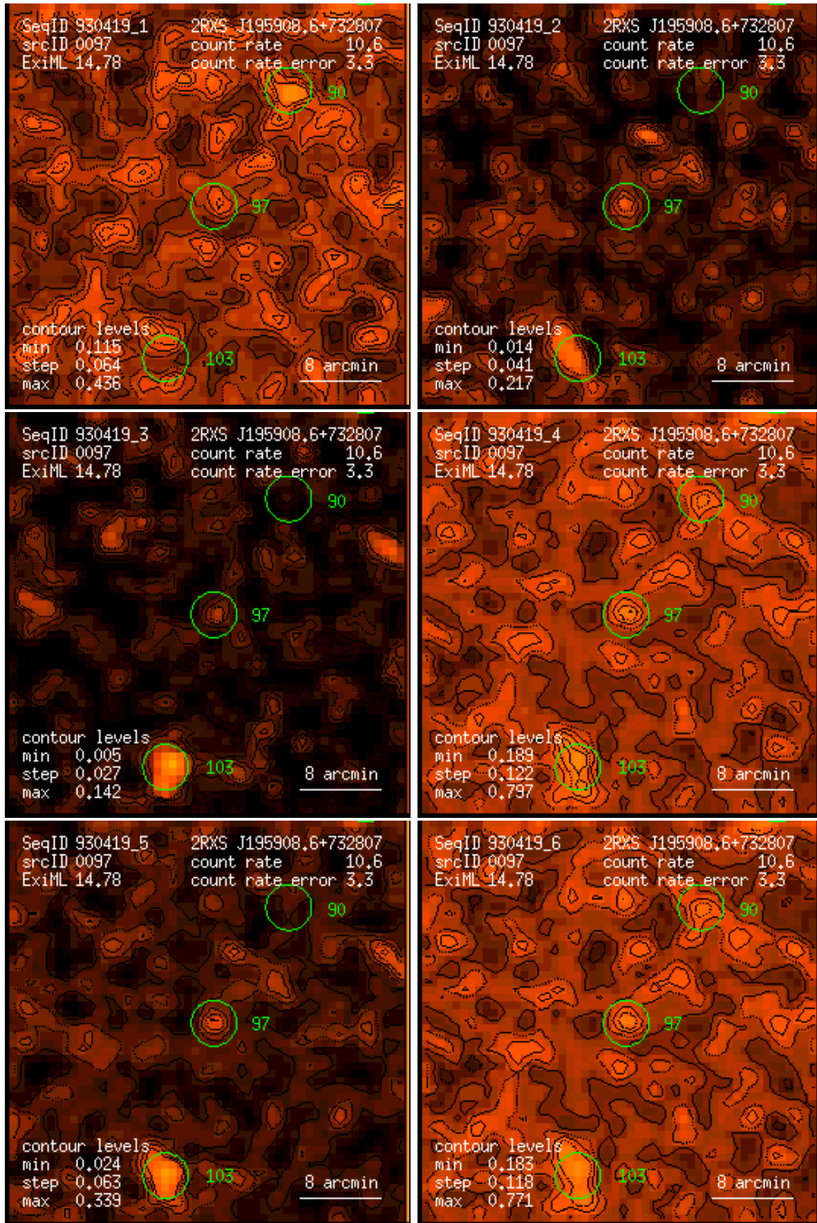
Figure 97: RASS 930419: detection 0097: band rate images, Gaussian filter: (1) PSPC channels 11 – 41, (2) 52 – 90, (3) 91 – 201, (4) 11 – 235, (5) 52 – 201, (6) 11 – 201. Broad band rates in counts/ks. Band rate contour levels in counts/ks/arcmin 2 .
