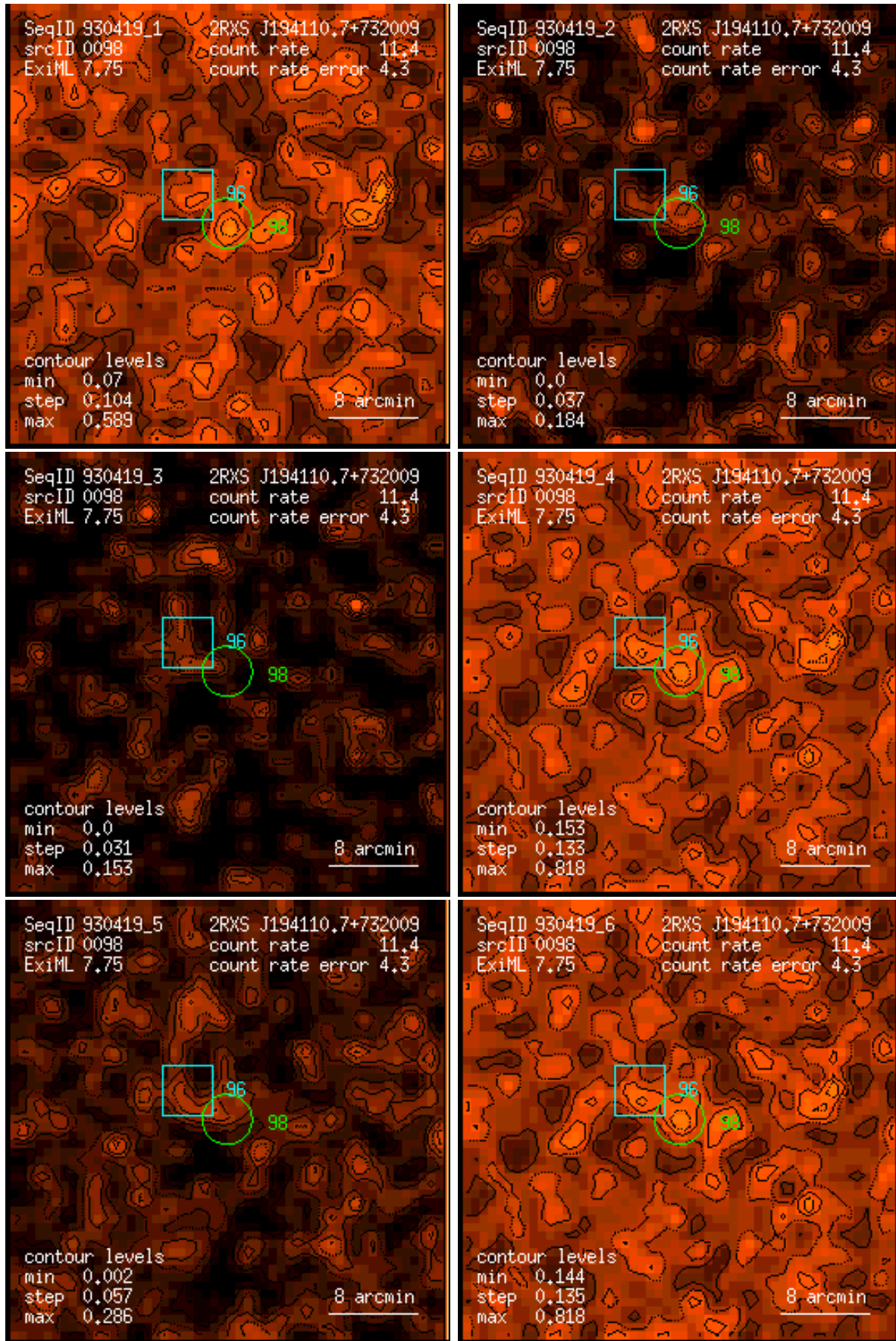
Figure 98: RASS 930419: detection 0098: band rate images, Gaussian filter: (1) PSPC channels 11 – 41, (2) 52 – 90, (3) 91 – 201, (4) 11 – 235, (5) 52 – 201, (6) 11 – 201. Broad band rates in counts/ks. Band rate contour levels in counts/ks/arcmin 2 .
