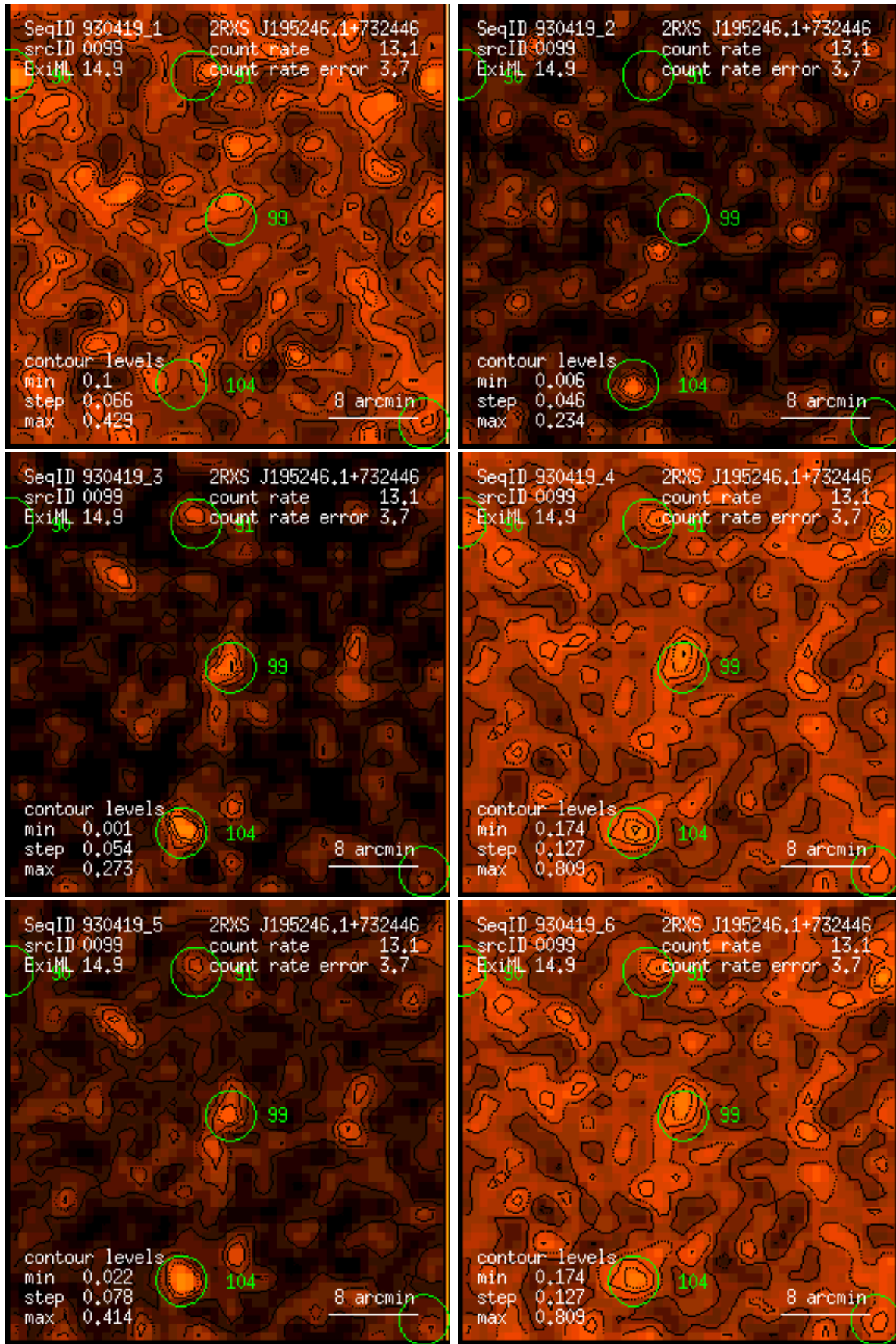
Figure 99: RASS 930419: detection 0099: band rate images, Gaussian filter: (1) PSPC channels 11 – 41, (2) 52 – 90, (3) 91 – 201, (4) 11 – 235, (5) 52 – 201, (6) 11 – 201. Broad band rates in counts/ks. Band rate contour levels in counts/ks/arcmin 2 .
