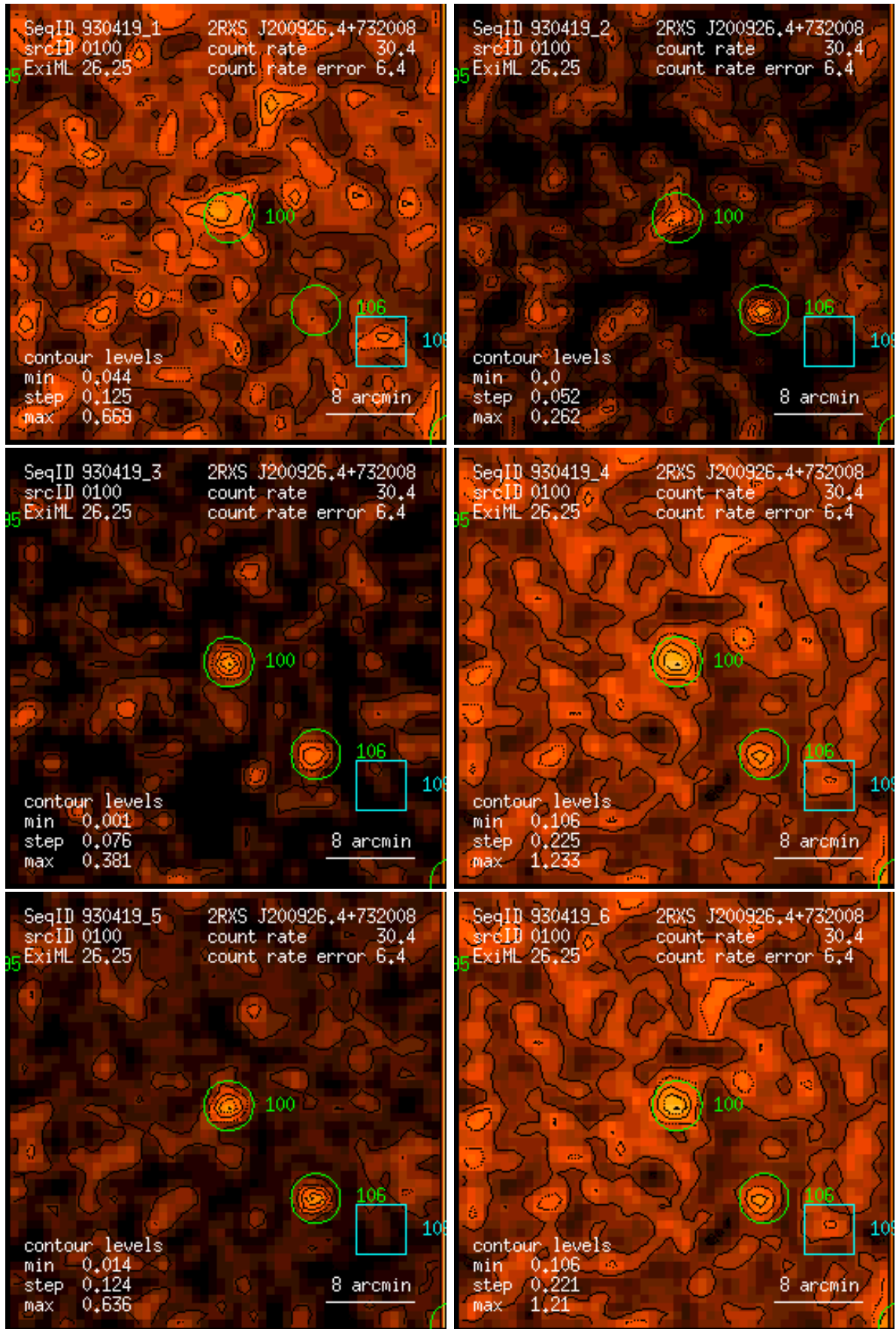
Figure 100: RASS 930419: detection 0100: band rate images, Gaussian filter: (1) PSPC channels 11 – 41, (2) 52 – 90, (3) 91 – 201, (4) 11 – 235, (5) 52 – 201, (6) 11 – 201. Broad band rates in counts/ks. Band rate contour levels in counts/ks/arcmin 2 .
