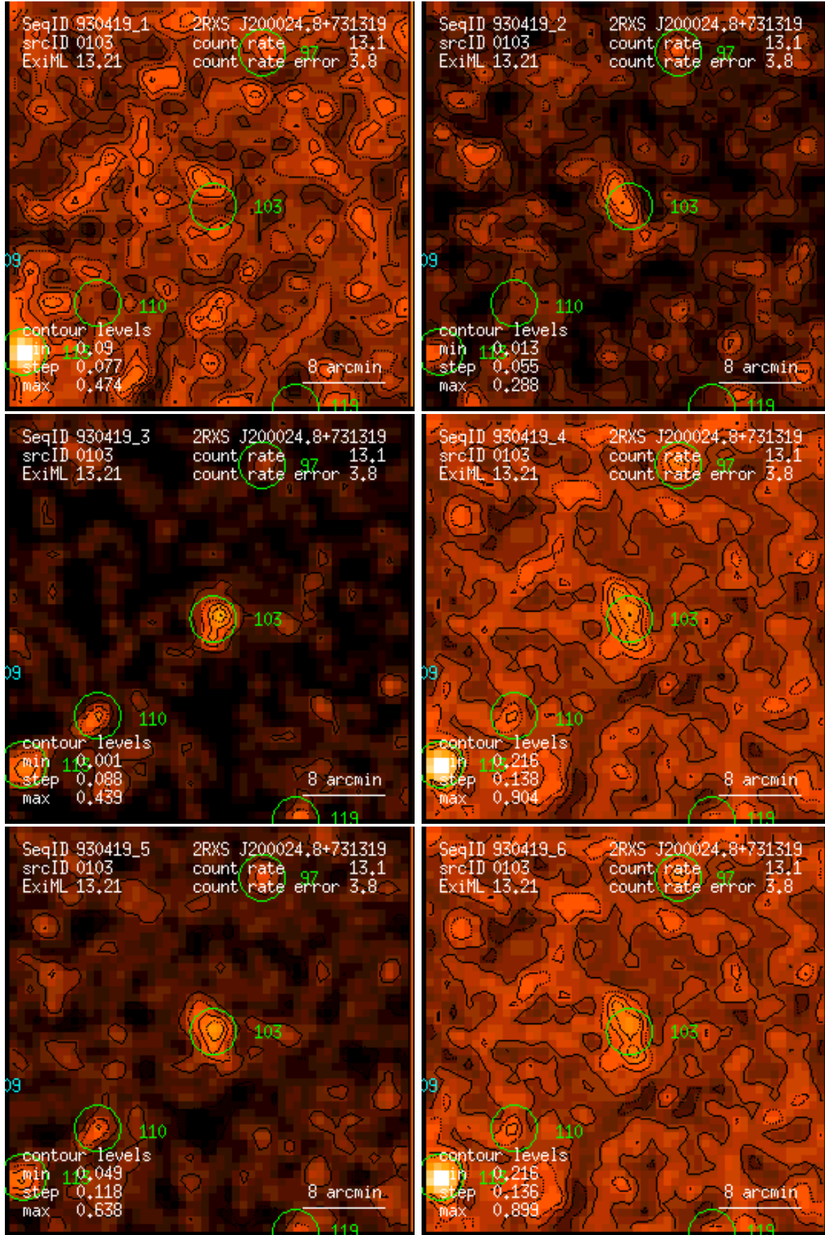
Figure 103: RASS 930419: detection 0103: band rate images, Gaussian filter: (1) PSPC channels 11 – 41, (2) 52 – 90, (3) 91 – 201, (4) 11 – 235, (5) 52 – 201, (6) 11 – 201. Broad band rates in counts/ks. Band rate contour levels in counts/ks/arcmin 2 .
