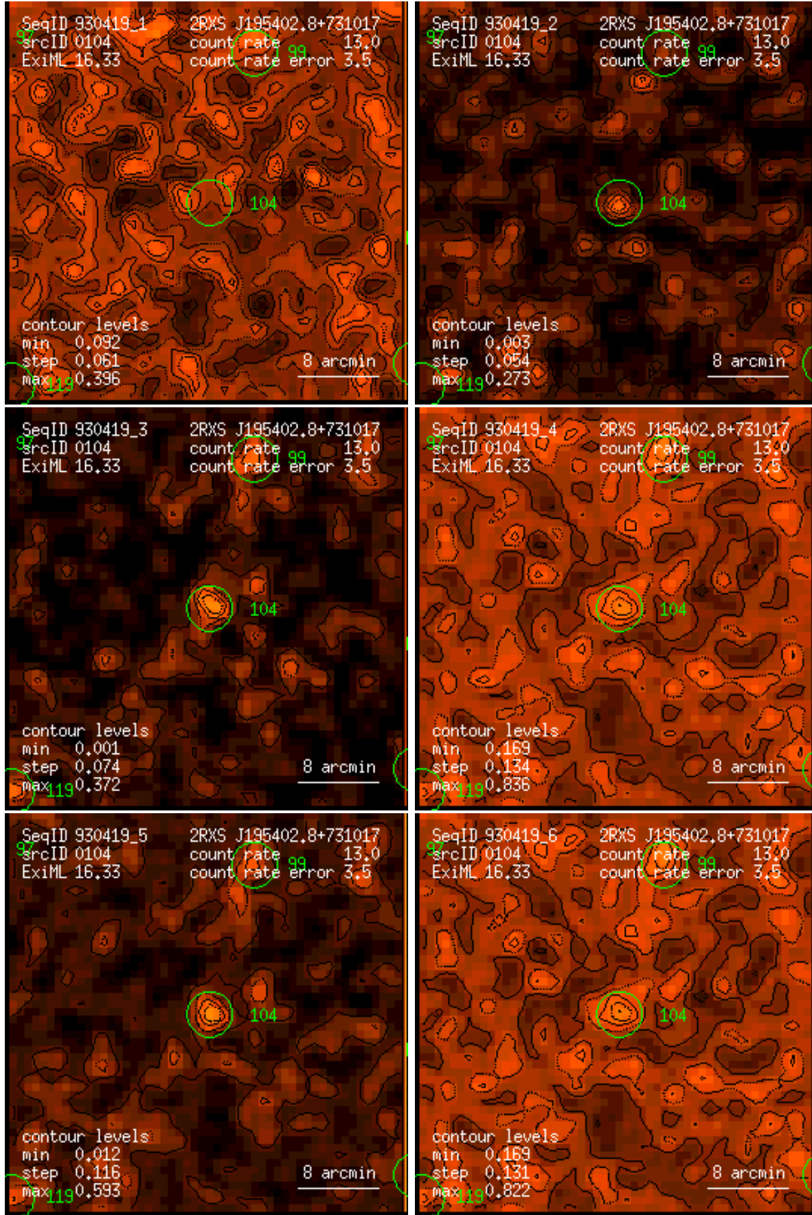
Figure 104: RASS 930419: detection 0104: band rate images, Gaussian filter: (1) PSPC channels 11 – 41, (2) 52 – 90, (3) 91 – 201, (4) 11 – 235, (5) 52 – 201, (6) 11 – 201. Broad band rates in counts/ks. Band rate contour levels in counts/ks/arcmin 2 .
