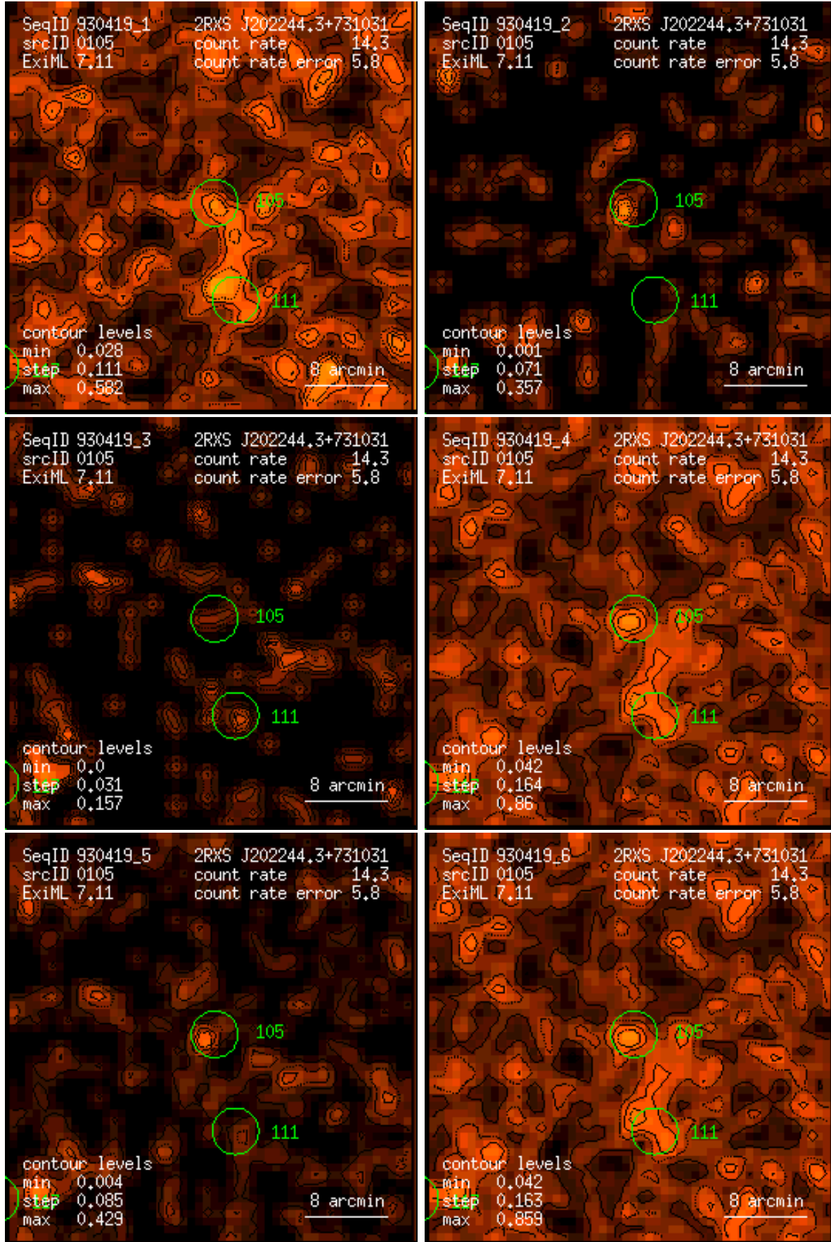
Figure 105: RASS 930419: detection 0105: band rate images, Gaussian filter: (1) PSPC channels 11 – 41, (2) 52 – 90, (3) 91 – 201, (4) 11 – 235, (5) 52 – 201, (6) 11 – 201. Broad band rates in counts/ks. Band rate contour levels in counts/ks/arcmin 2 .
