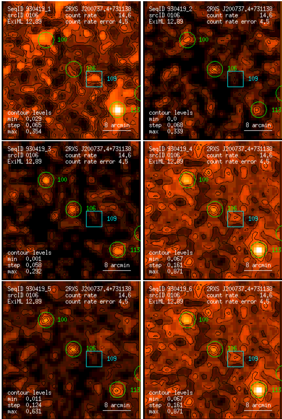
Figure 106: RASS 930419: detection 0106: band rate images, Gaussian filter: (1) PSPC channels 11 – 41, (2) 52 – 90, (3) 91 – 201, (4) 11 – 235, (5) 52 – 201, (6) 11 – 201. Broad band rates in counts/ks. Band rate contour levels in counts/ks/arcmin 2 .
