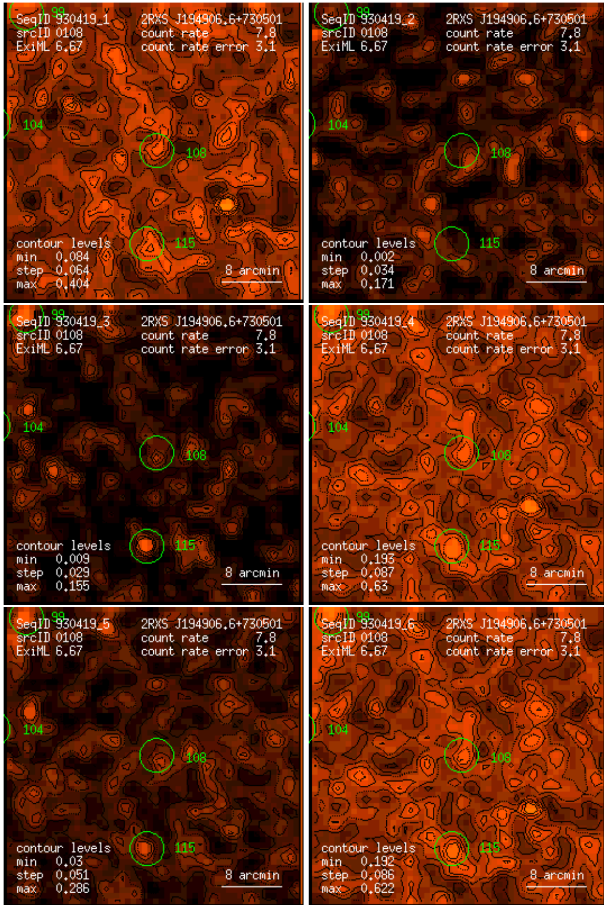
Figure 108: RASS 930419: detection 0108: band rate images, Gaussian filter: (1) PSPC channels 11 – 41, (2) 52 – 90, (3) 91 – 201, (4) 11 – 235, (5) 52 – 201, (6) 11 – 201. Broad band rates in counts/ks. Band rate contour levels in counts/ks/arcmin 2 .
