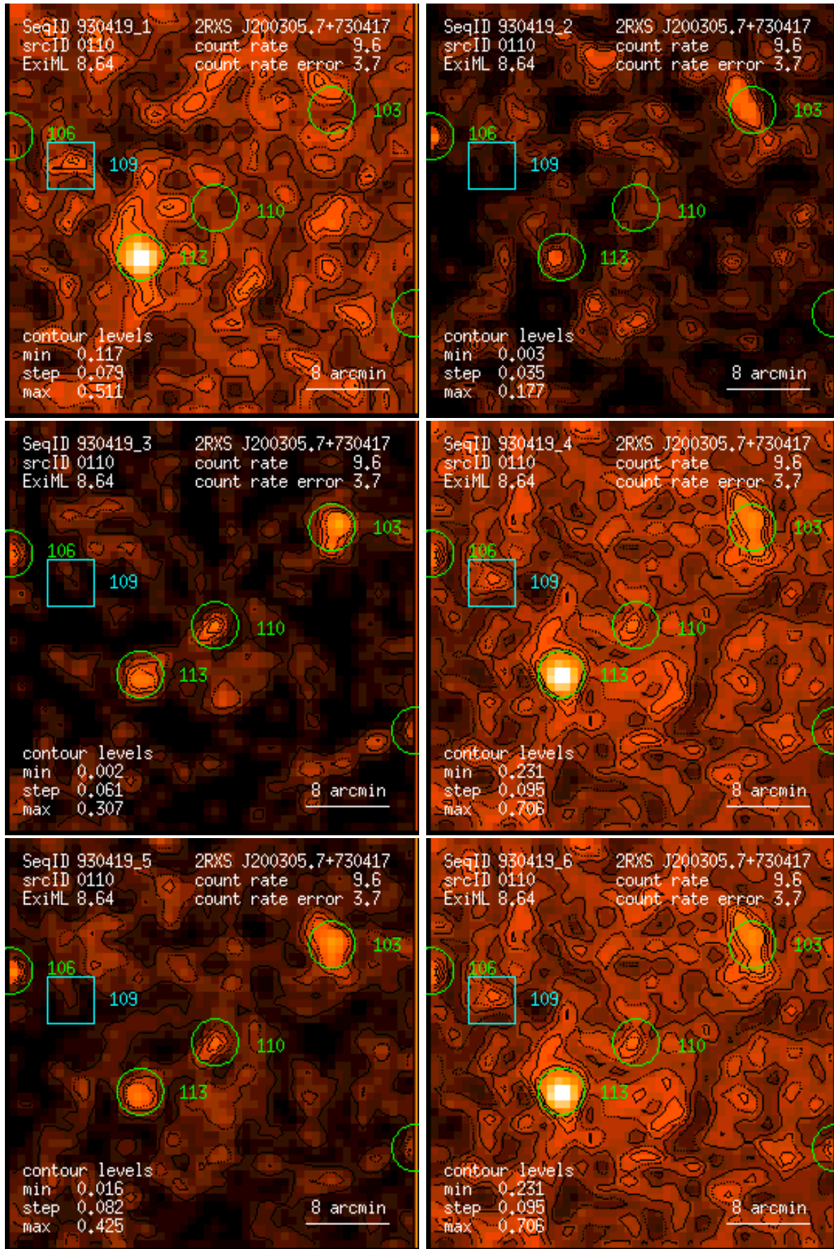
Figure 110: RASS 930419: detection 0110: band rate images, Gaussian filter: (1) PSPC channels 11 – 41, (2) 52 – 90, (3) 91 – 201, (4) 11 – 235, (5) 52 – 201, (6) 11 – 201. Broad band rates in counts/ks. Band rate contour levels in counts/ks/arcmin 2 .
