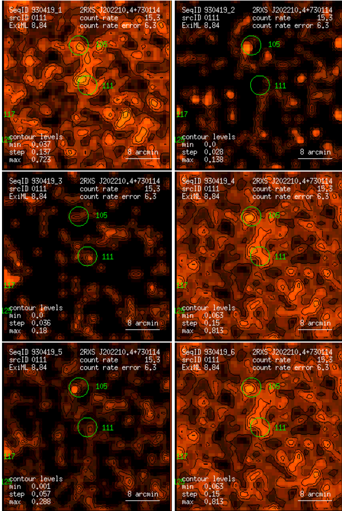
Figure 111: RASS 930419: detection 0111: band rate images, Gaussian filter: (1) PSPC channels 11 – 41, (2) 52 – 90, (3) 91 – 201, (4) 11 – 235, (5) 52 – 201, (6) 11 – 201. Broad band rates in counts/ks. Band rate contour levels in counts/ks/arcmin 2 .
