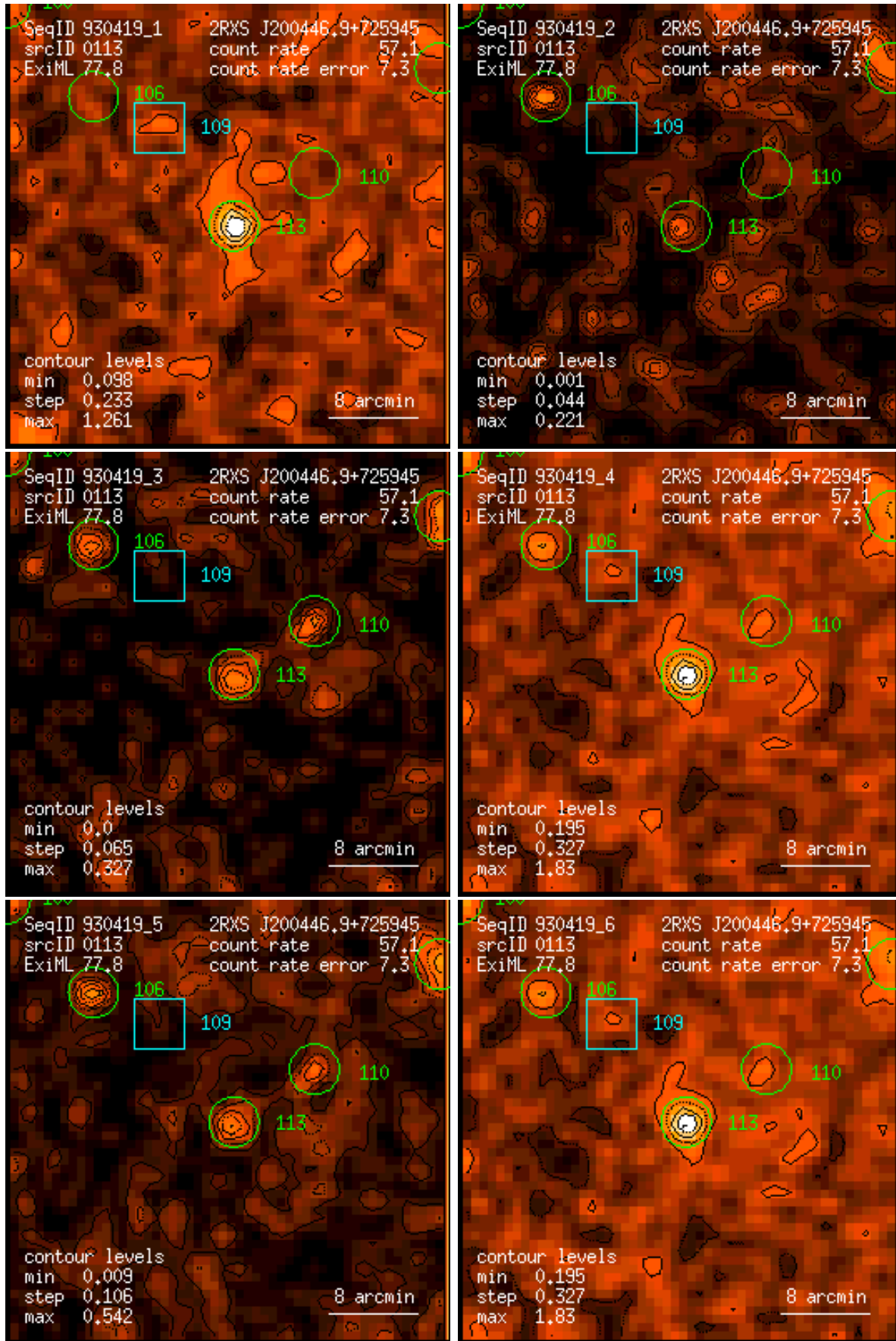
Figure 113: RASS 930419: detection 0113: band rate images, Gaussian filter: (1) PSPC channels 11 – 41, (2) 52 – 90, (3) 91 – 201, (4) 11 – 235, (5) 52 – 201, (6) 11 – 201. Broad band rates in counts/ks. Band rate contour levels in counts/ks/arcmin 2 .
