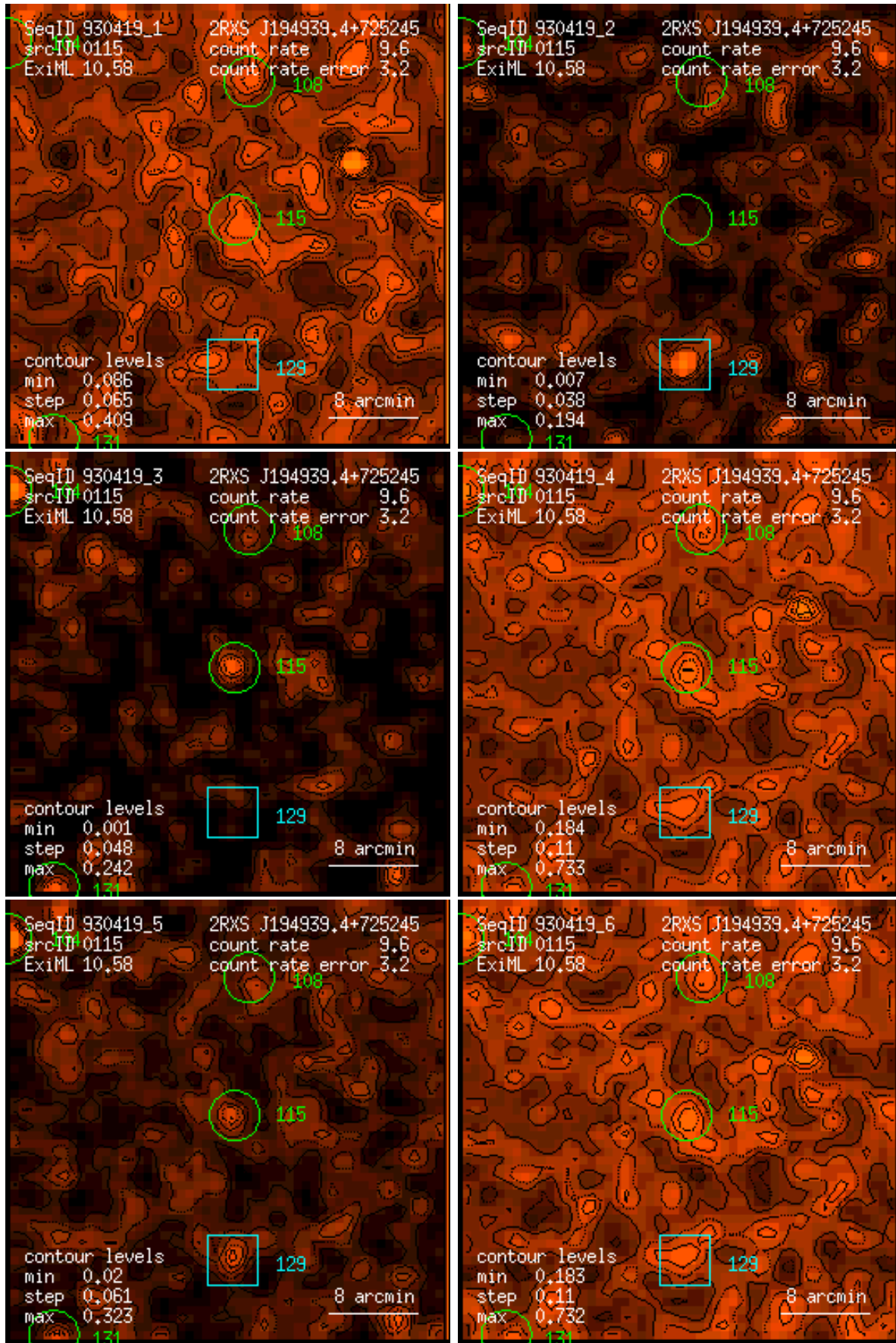
Figure 115: RASS 930419: detection 0115: band rate images, Gaussian filter: (1) PSPC channels 11 – 41, (2) 52 – 90, (3) 91 – 201, (4) 11 – 235, (5) 52 – 201, (6) 11 – 201. Broad band rates in counts/ks. Band rate contour levels in counts/ks/arcmin 2 .
