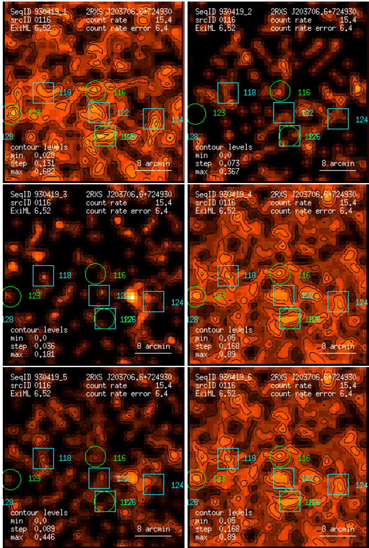
Figure 116: RASS 930419: detection 0116: band rate images, Gaussian filter: (1) PSPC channels 11 – 41, (2) 52 – 90, (3) 91 – 201, (4) 11 – 235, (5) 52 – 201, (6) 11 – 201. Broad band rates in counts/ks. Band rate contour levels in counts/ks/arcmin 2 .
