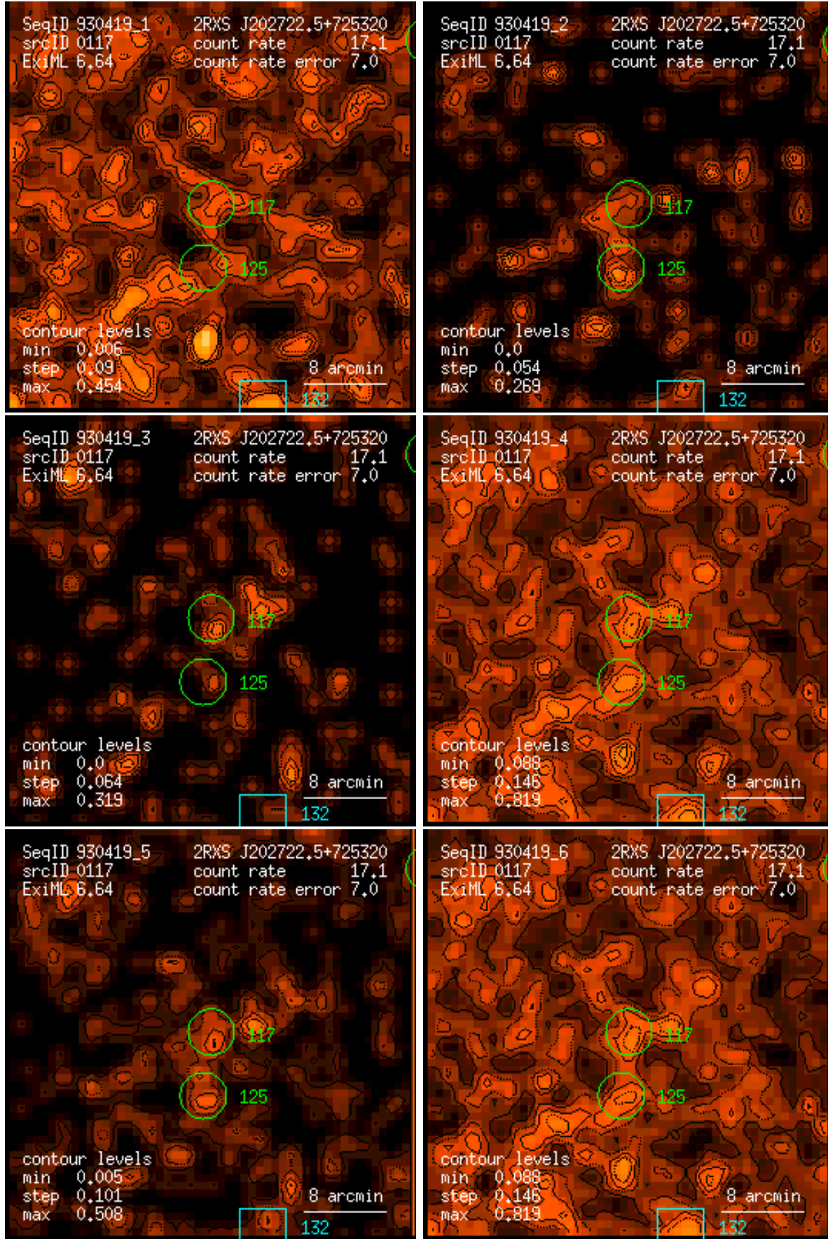
Figure 117: RASS 930419: detection 0117: band rate images, Gaussian filter: (1) PSPC channels 11 – 41, (2) 52 – 90, (3) 91 – 201, (4) 11 – 235, (5) 52 – 201, (6) 11 – 201. Broad band rates in counts/ks. Band rate contour levels in counts/ks/arcmin 2 .
