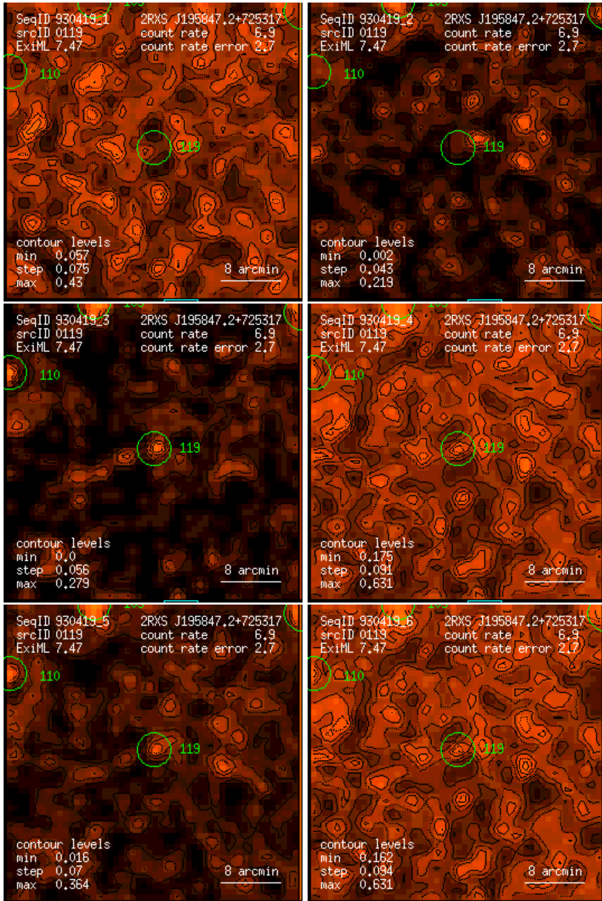
Figure 119: RASS 930419: detection 0119: band rate images, Gaussian filter: (1) PSPC channels 11 – 41, (2) 52 – 90, (3) 91 – 201, (4) 11 – 235, (5) 52 – 201, (6) 11 – 201. Broad band rates in counts/ks. Band rate contour levels in counts/ks/arcmin 2 .
