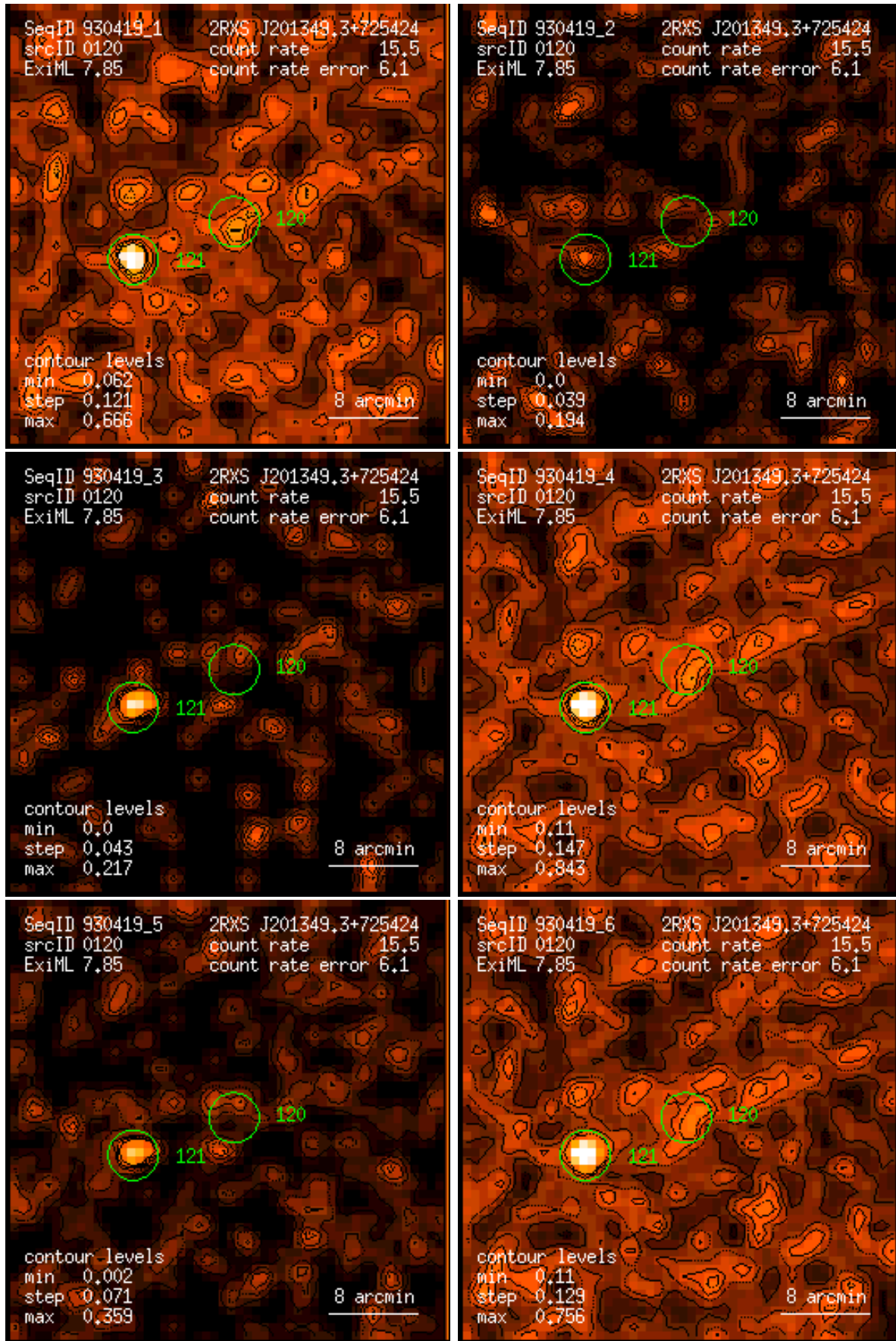
Figure 120: RASS 930419: detection 0120: band rate images, Gaussian filter: (1) PSPC channels 11 – 41, (2) 52 – 90, (3) 91 – 201, (4) 11 – 235, (5) 52 – 201, (6) 11 – 201. Broad band rates in counts/ks. Band rate contour levels in counts/ks/arcmin 2 .
