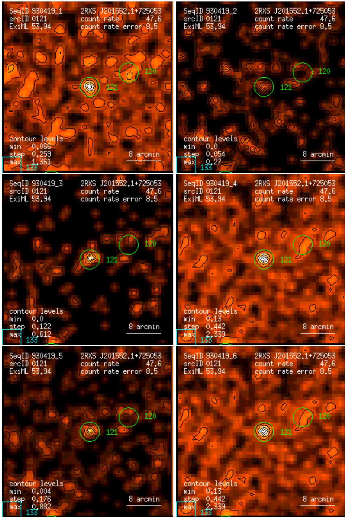
Figure 121: RASS 930419: detection 0121: band rate images, Gaussian filter: (1) PSPC channels 11 – 41, (2) 52 – 90, (3) 91 – 201, (4) 11 – 235, (5) 52 – 201, (6) 11 – 201. Broad band rates in counts/ks. Band rate contour levels in counts/ks/arcmin 2 .
