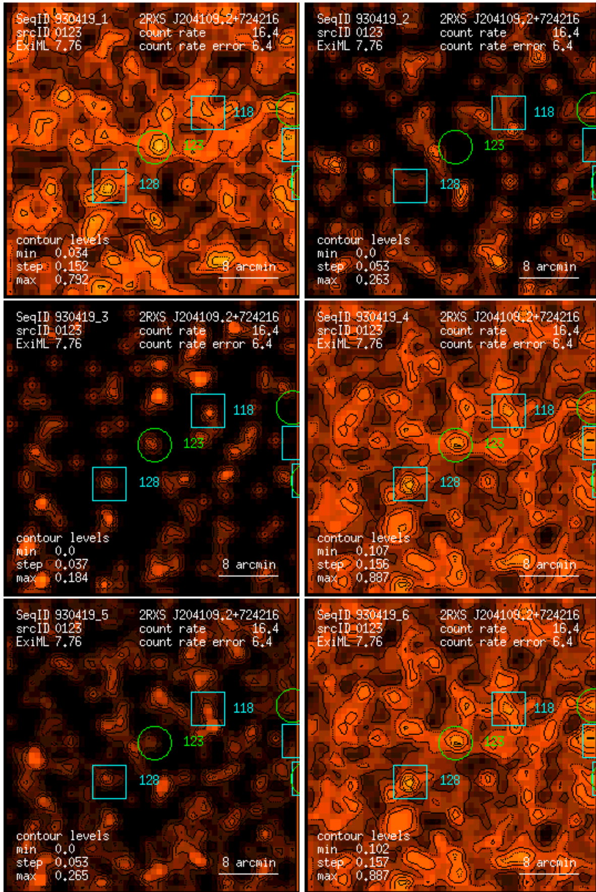
Figure 123: RASS 930419: detection 0123: band rate images, Gaussian filter: (1) PSPC channels 11 – 41, (2) 52 – 90, (3) 91 – 201, (4) 11 – 235, (5) 52 – 201, (6) 11 – 201. Broad band rates in counts/ks. Band rate contour levels in counts/ks/arcmin 2 .
