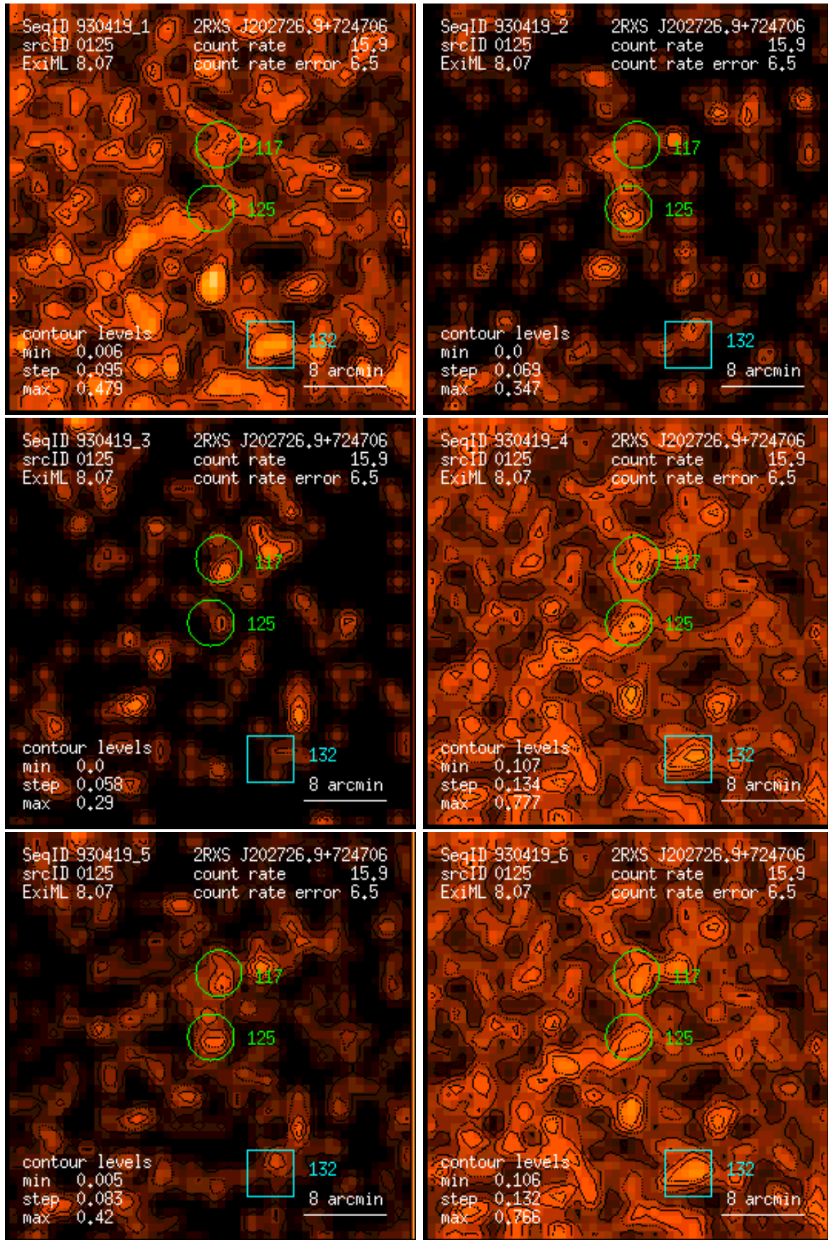
Figure 125: RASS 930419: detection 0125: band rate images, Gaussian filter: (1) PSPC channels 11 – 41, (2) 52 – 90, (3) 91 – 201, (4) 11 – 235, (5) 52 – 201, (6) 11 – 201. Broad band rates in counts/ks. Band rate contour levels in counts/ks/arcmin 2 .
