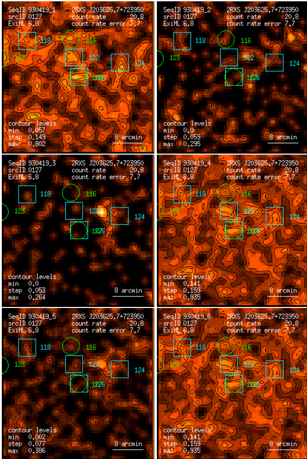
Figure 127: RASS 930419: detection 0127: band rate images, Gaussian filter: (1) PSPC channels 11 – 41, (2) 52 – 90, (3) 91 – 201, (4) 11 – 235, (5) 52 – 201, (6) 11 – 201. Broad band rates in counts/ks. Band rate contour levels in counts/ks/arcmin 2 .
