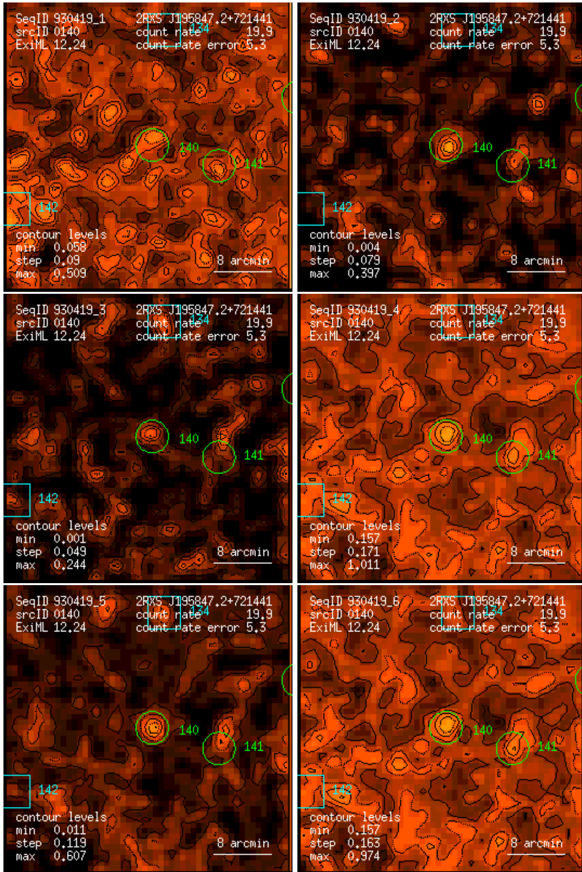
Figure 140: RASS 930419: detection 0140: band rate images, Gaussian filter: (1) PSPC channels 11 – 41, (2) 52 – 90, (3) 91 – 201, (4) 11 – 235, (5) 52 – 201, (6) 11 – 201. Broad band rates in counts/ks. Band rate contour levels in counts/ks/arcmin 2 .
