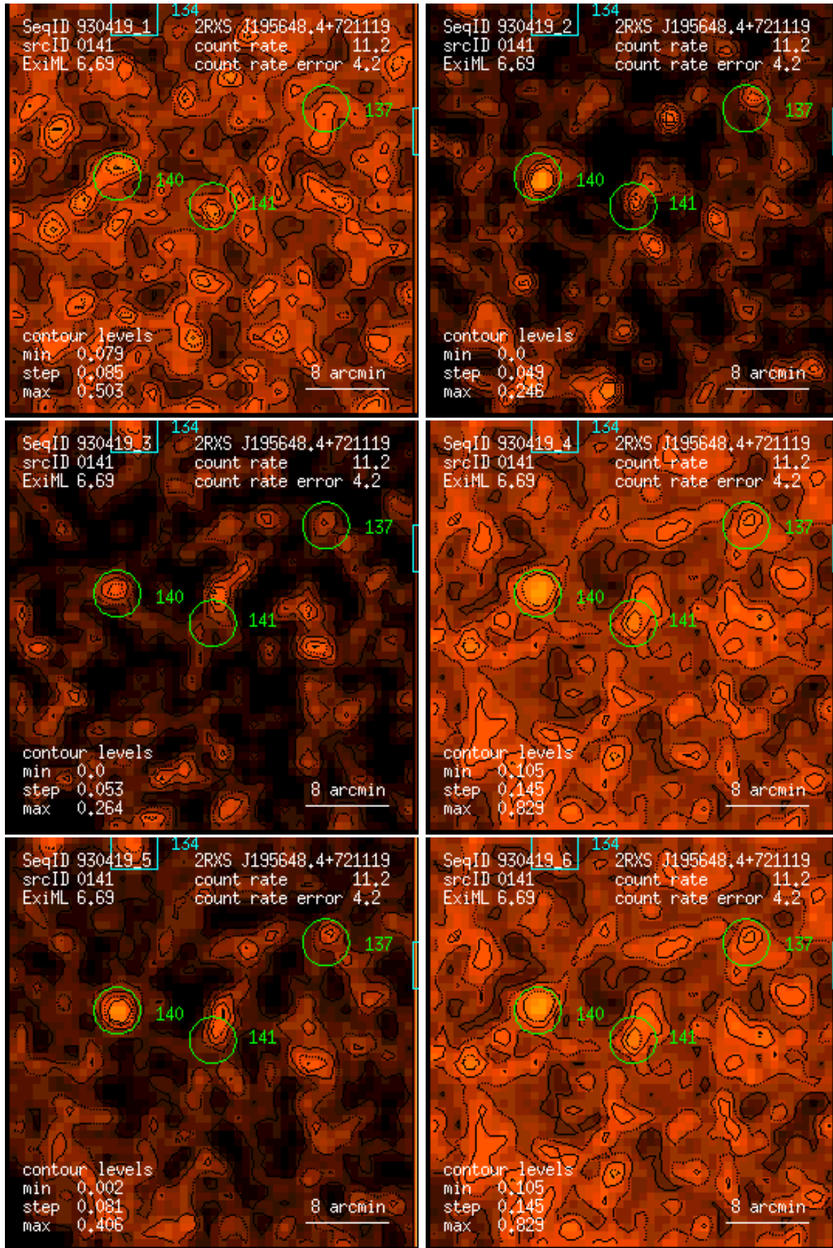
Figure 141: RASS 930419: detection 0141: band rate images, Gaussian filter: (1) PSPC channels 11 – 41, (2) 52 – 90, (3) 91 – 201, (4) 11 – 235, (5) 52 – 201, (6) 11 – 201. Broad band rates in counts/ks. Band rate contour levels in counts/ks/arcmin 2 .
