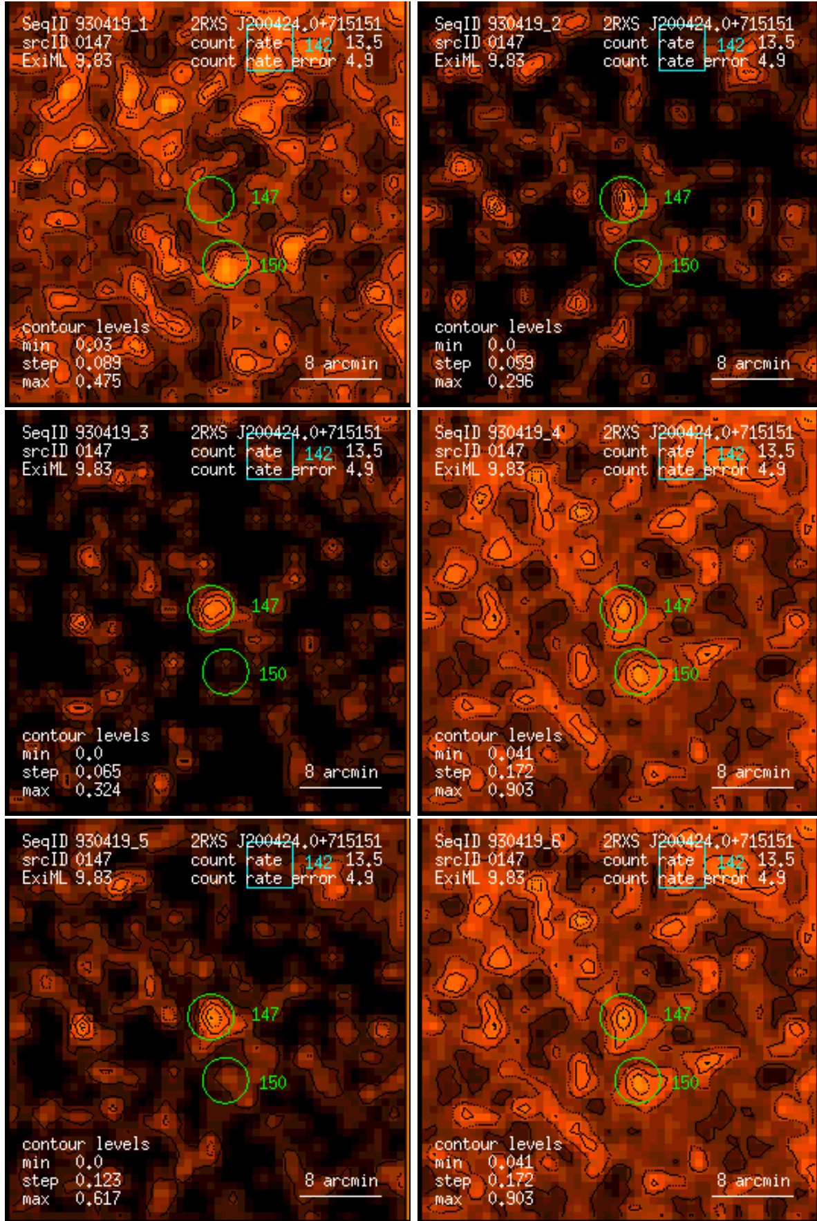
Figure 147: RASS 930419: detection 0147: band rate images, Gaussian filter: (1) PSPC channels 11 – 41, (2) 52 – 90, (3) 91 – 201, (4) 11 – 235, (5) 52 – 201, (6) 11 – 201. Broad band rates in counts/ks. Band rate contour levels in counts/ks/arcmin 2 .
