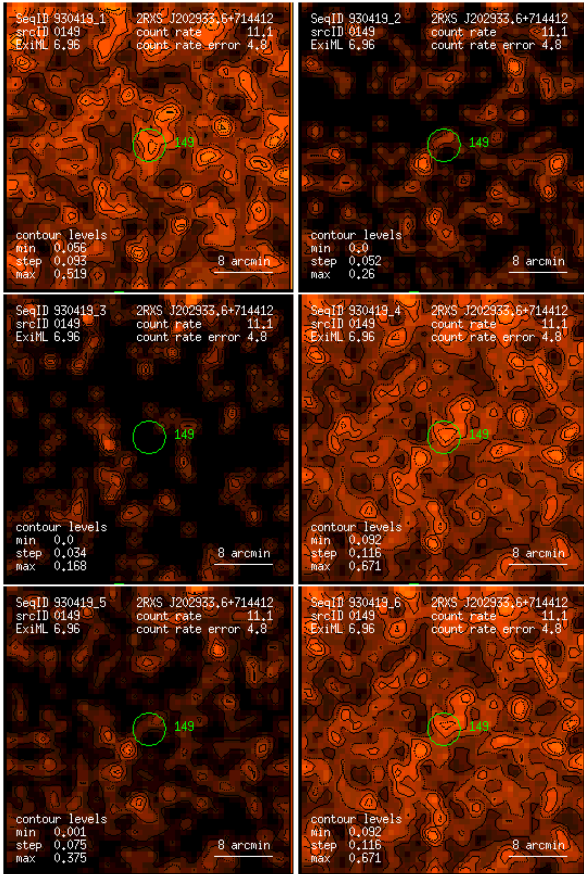
Figure 149: RASS 930419: detection 0149: band rate images, Gaussian filter: (1) PSPC channels 11 – 41, (2) 52 – 90, (3) 91 – 201, (4) 11 – 235, (5) 52 – 201, (6) 11 – 201. Broad band rates in counts/ks. Band rate contour levels in counts/ks/arcmin 2 .
