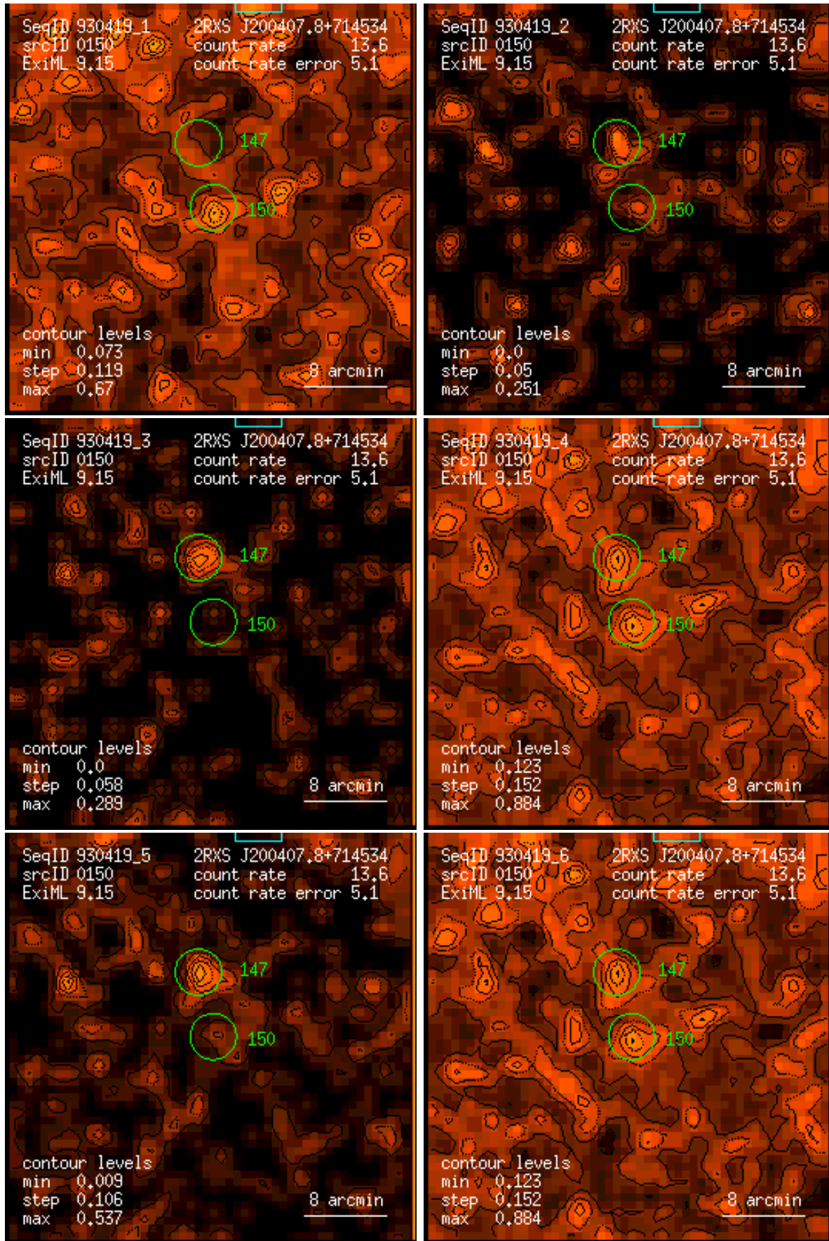
Figure 150: RASS 930419: detection 0150: band rate images, Gaussian filter: (1) PSPC channels 11 – 41, (2) 52 – 90, (3) 91 – 201, (4) 11 – 235, (5) 52 – 201, (6) 11 – 201. Broad band rates in counts/ks. Band rate contour levels in counts/ks/arcmin 2 .
