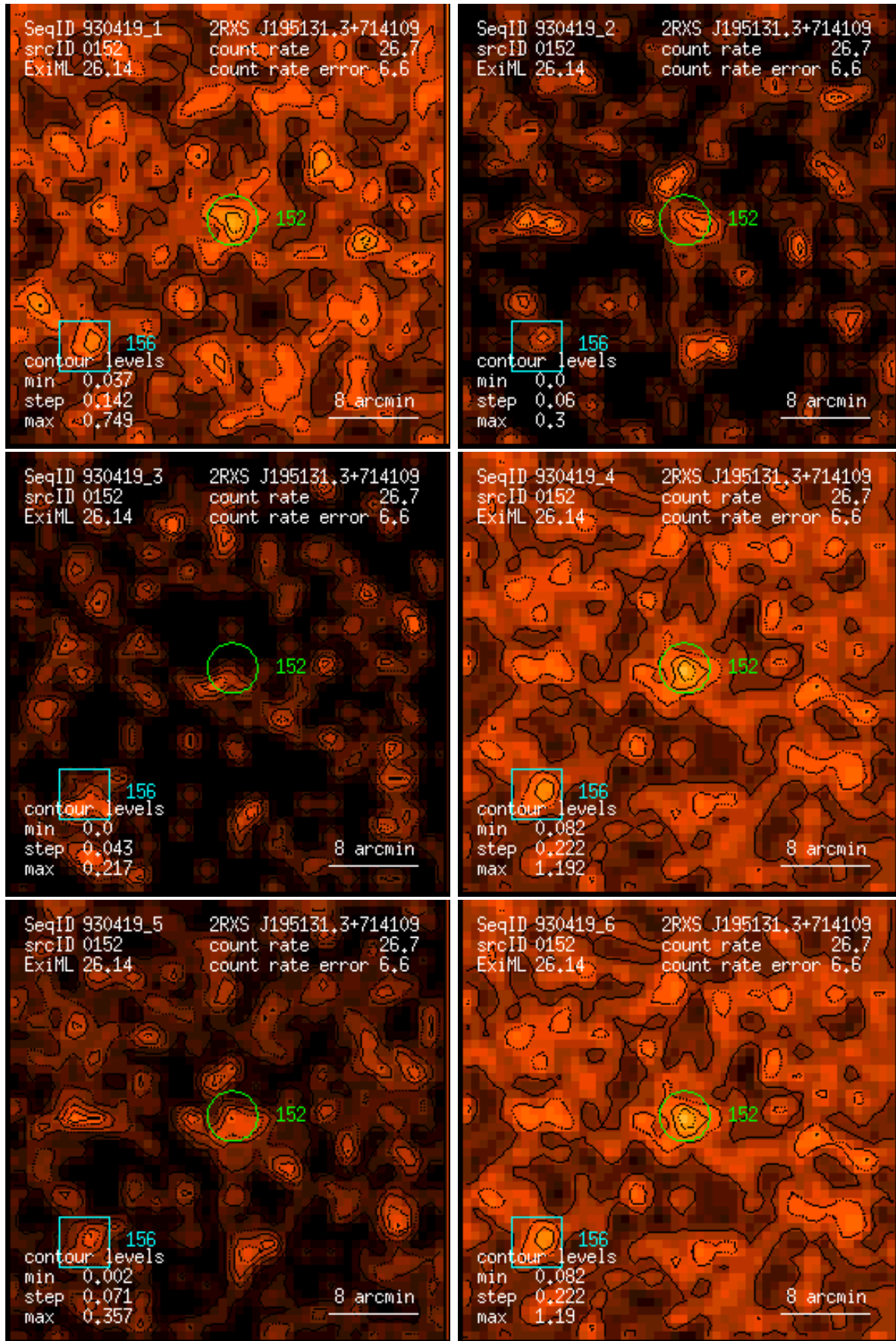
Figure 152: RASS 930419: detection 0152: band rate images, Gaussian filter: (1) PSPC channels 11 – 41, (2) 52 – 90, (3) 91 – 201, (4) 11 – 235, (5) 52 – 201, (6) 11 – 201. Broad band rates in counts/ks. Band rate contour levels in counts/ks/arcmin 2 .
