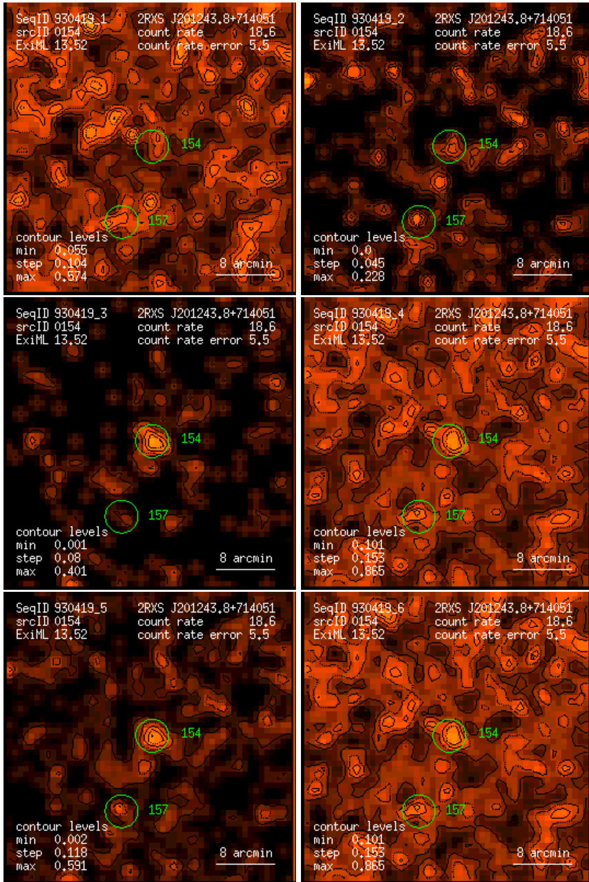
Figure 154: RASS 930419: detection 0154: band rate images, Gaussian filter: (1) PSPC channels 11 – 41, (2) 52 – 90, (3) 91 – 201, (4) 11 – 235, (5) 52 – 201, (6) 11 – 201. Broad band rates in counts/ks. Band rate contour levels in counts/ks/arcmin 2 .
