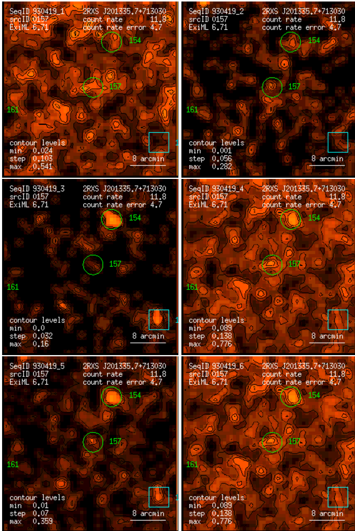
Figure 157: RASS 930419: detection 0157: band rate images, Gaussian filter: (1) PSPC channels 11 – 41, (2) 52 – 90, (3) 91 – 201, (4) 11 – 235, (5) 52 – 201, (6) 11 – 201. Broad band rates in counts/ks. Band rate contour levels in counts/ks/arcmin 2 .
