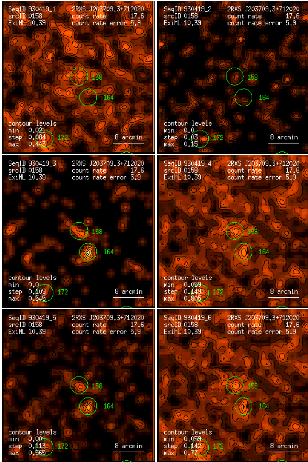
Figure 158: RASS 930419: detection 0158: band rate images, Gaussian filter: (1) PSPC channels 11 – 41, (2) 52 – 90, (3) 91 – 201, (4) 11 – 235, (5) 52 – 201, (6) 11 – 201. Broad band rates in counts/ks. Band rate contour levels in counts/ks/arcmin 2 .
