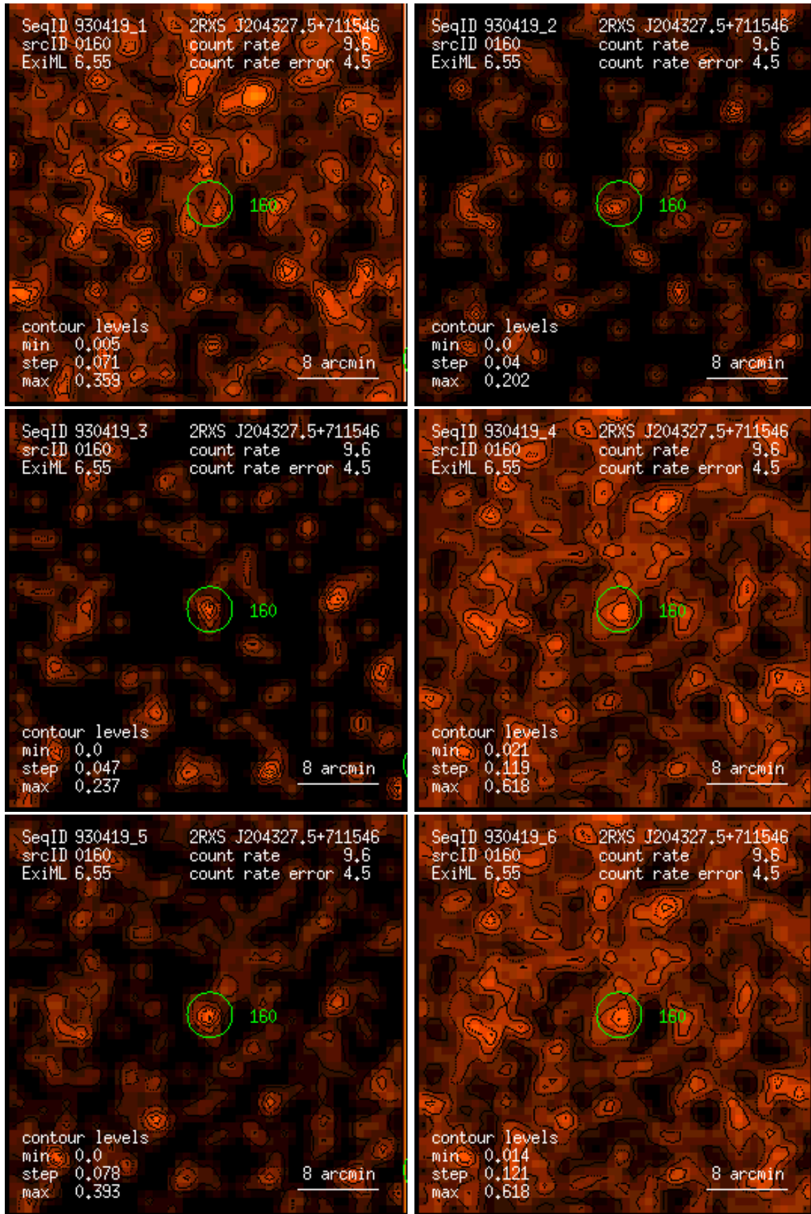
Figure 160: RASS 930419: detection 0160: band rate images, Gaussian filter: (1) PSPC channels 11 – 41, (2) 52 – 90, (3) 91 – 201, (4) 11 – 235, (5) 52 – 201, (6) 11 – 201. Broad band rates in counts/ks. Band rate contour levels in counts/ks/arcmin 2 .
