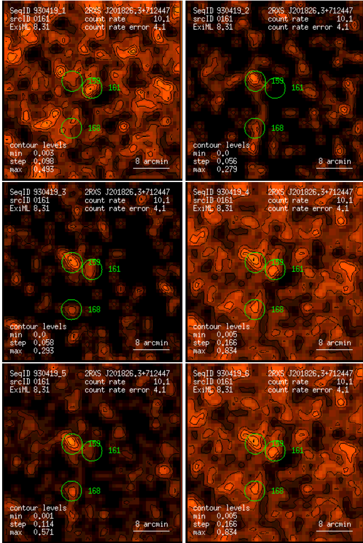
Figure 161: RASS 930419: detection 0161: band rate images, Gaussian filter: (1) PSPC channels 11 – 41, (2) 52 – 90, (3) 91 – 201, (4) 11 – 235, (5) 52 – 201, (6) 11 – 201. Broad band rates in counts/ks. Band rate contour levels in counts/ks/arcmin 2 .
