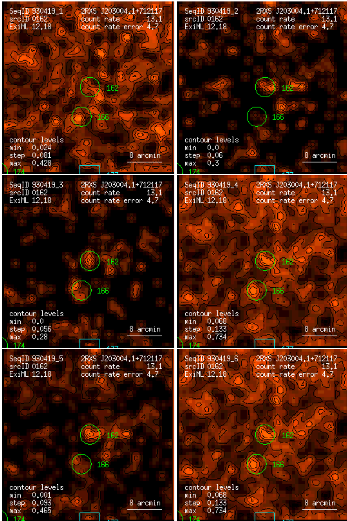
Figure 162: RASS 930419: detection 0162: band rate images, Gaussian filter: (1) PSPC channels 11 – 41, (2) 52 – 90, (3) 91 – 201, (4) 11 – 235, (5) 52 – 201, (6) 11 – 201. Broad band rates in counts/ks. Band rate contour levels in counts/ks/arcmin 2 .
