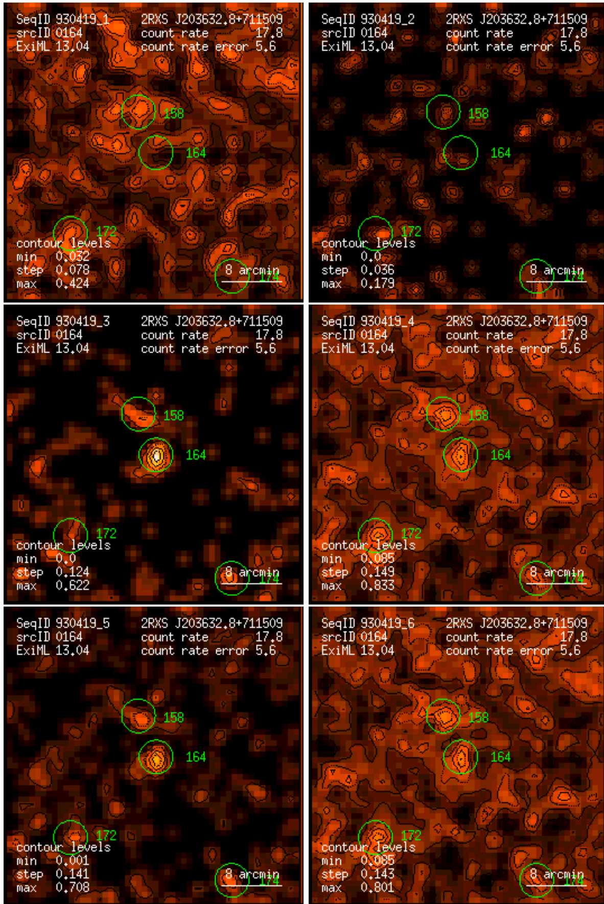
Figure 164: RASS 930419: detection 0164: band rate images, Gaussian filter: (1) PSPC channels 11 – 41, (2) 52 – 90, (3) 91 – 201, (4) 11 – 235, (5) 52 – 201, (6) 11 – 201. Broad band rates in counts/ks. Band rate contour levels in counts/ks/arcmin 2 .
