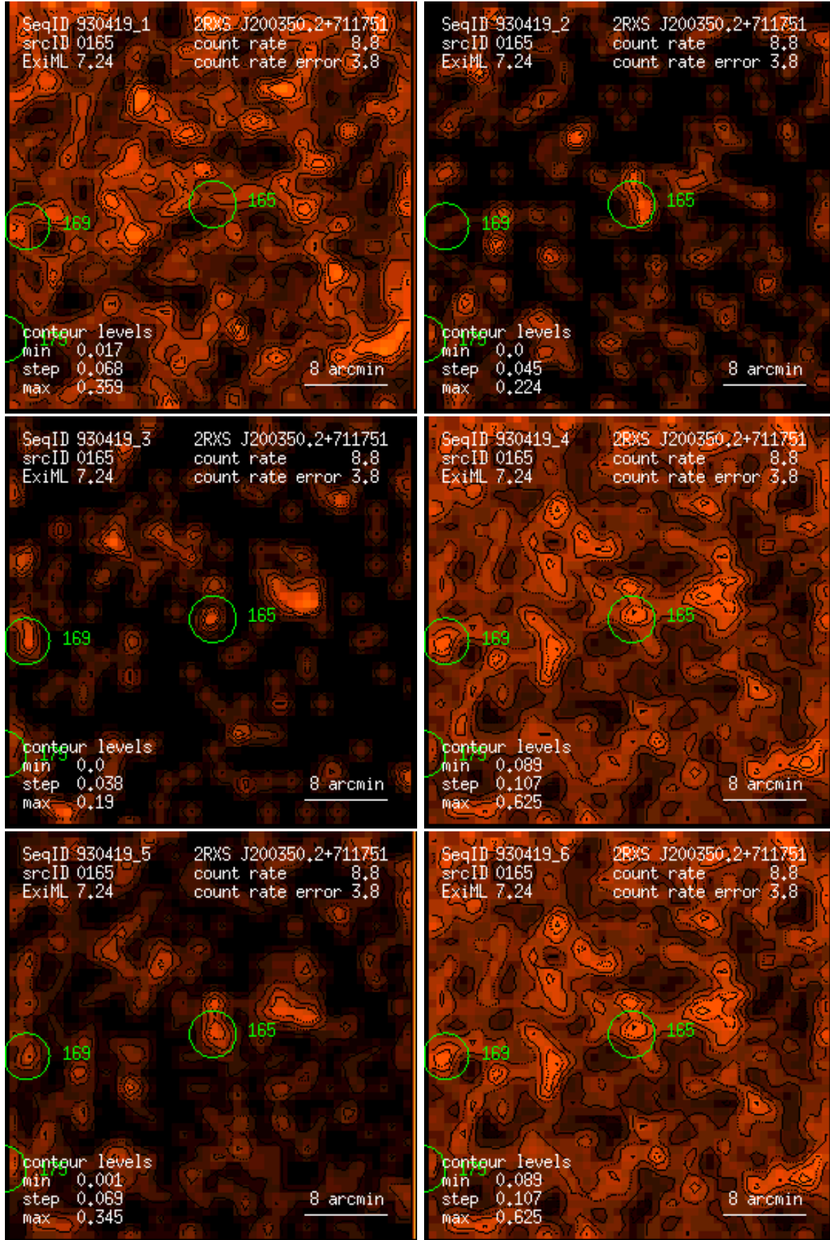
Figure 165: RASS 930419: detection 0165: band rate images, Gaussian filter: (1) PSPC channels 11 – 41, (2) 52 – 90, (3) 91 – 201, (4) 11 – 235, (5) 52 – 201, (6) 11 – 201. Broad band rates in counts/ks. Band rate contour levels in counts/ks/arcmin 2 .
