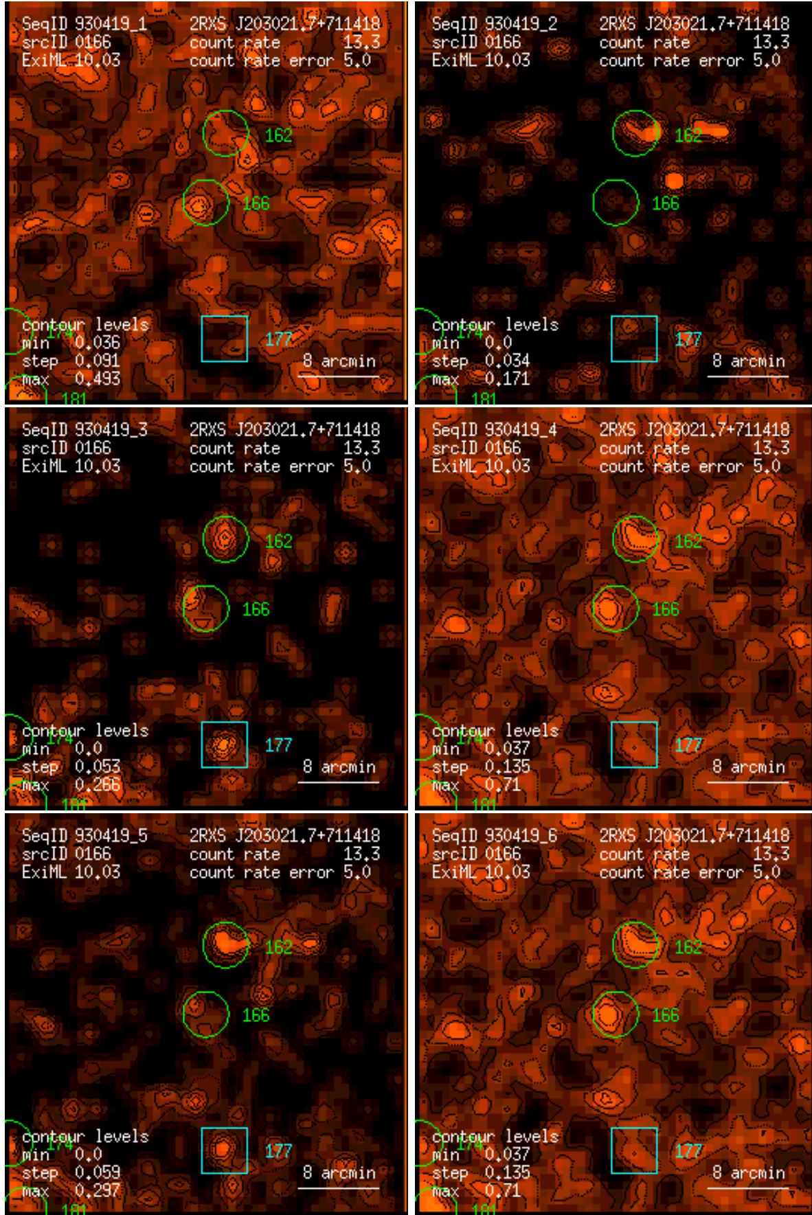
Figure 166: RASS 930419: detection 0166: band rate images, Gaussian filter: (1) PSPC channels 11 – 41, (2) 52 – 90, (3) 91 – 201, (4) 11 – 235, (5) 52 – 201, (6) 11 – 201. Broad band rates in counts/ks. Band rate contour levels in counts/ks/arcmin 2 .
