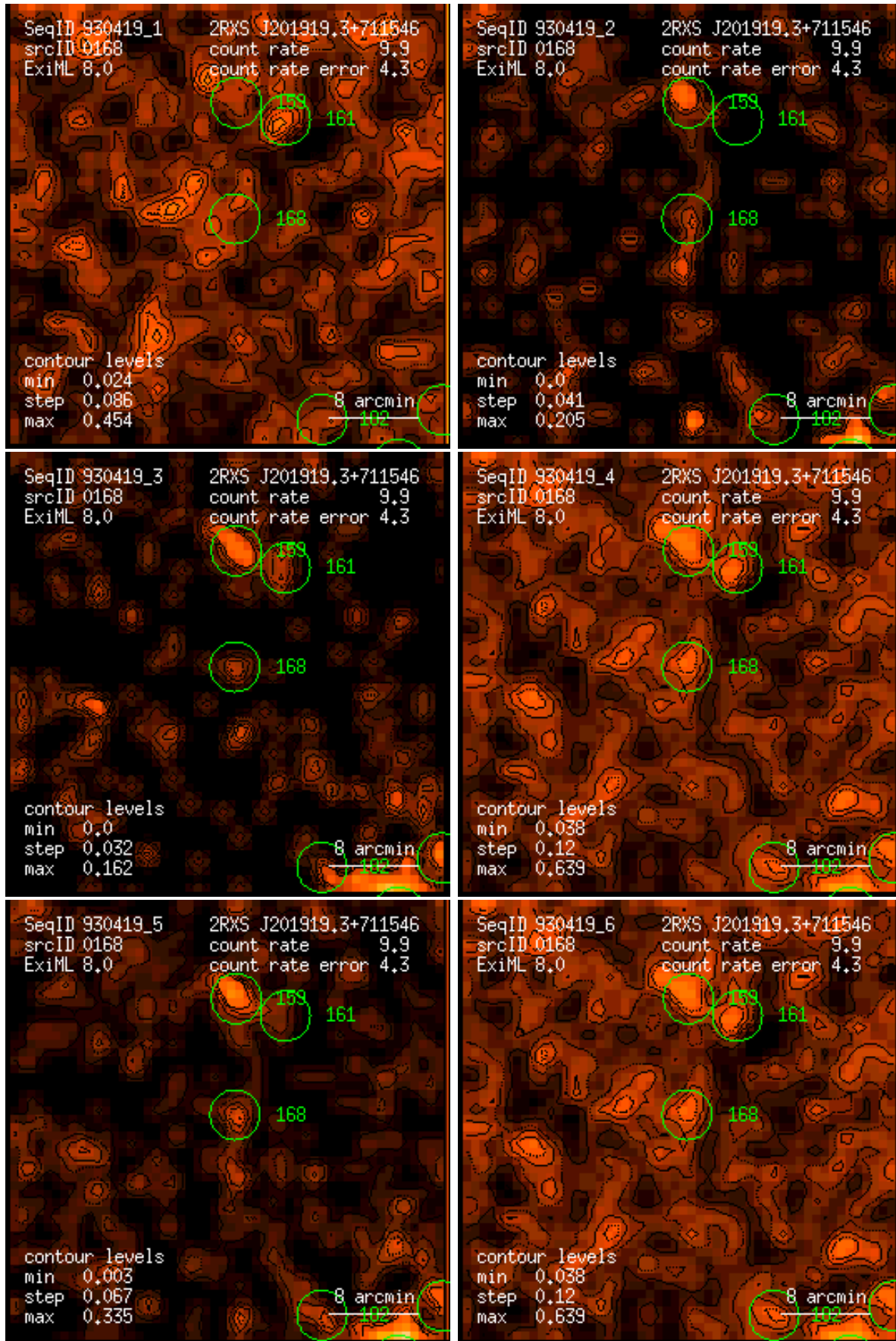
Figure 168: RASS 930419: detection 0168: band rate images, Gaussian filter: (1) PSPC channels 11 – 41, (2) 52 – 90, (3) 91 – 201, (4) 11 – 235, (5) 52 – 201, (6) 11 – 201. Broad band rates in counts/ks. Band rate contour levels in counts/ks/arcmin 2 .
